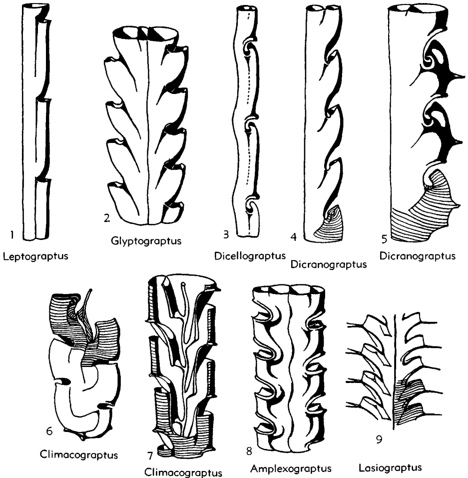
FIG. 31. Variations in graptolite thecae, mostly somewhat diagrammatic (8). 1, Leptograptus , \times 15 . 2, Glyptograptus , \times 15 . 3, Dicellograptus geniculatus , \times 19 . 4, Dicranograptus pringlei , \times 11 . 5, Dicranograptus nicholsoni , \times 11 . 6, Climacograptus scharenbergi , \times 22 . 7, Climacograptus typicalis , \times 19 . 8, Amplexograptus cf. coelatus , \times 13 . 9, Lasiograptus harknessi , \times 10 .
