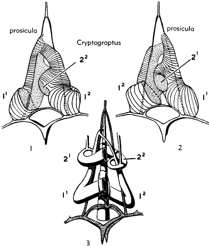
FIG. 44. Cryptograptid development illustrated by very early growth stage of Cryptograptus tricornis X20 (9). 1, Reverse view. 2, Obverse view, with thecal diagram and clathrial framework. Growth lines slightly schematic.
