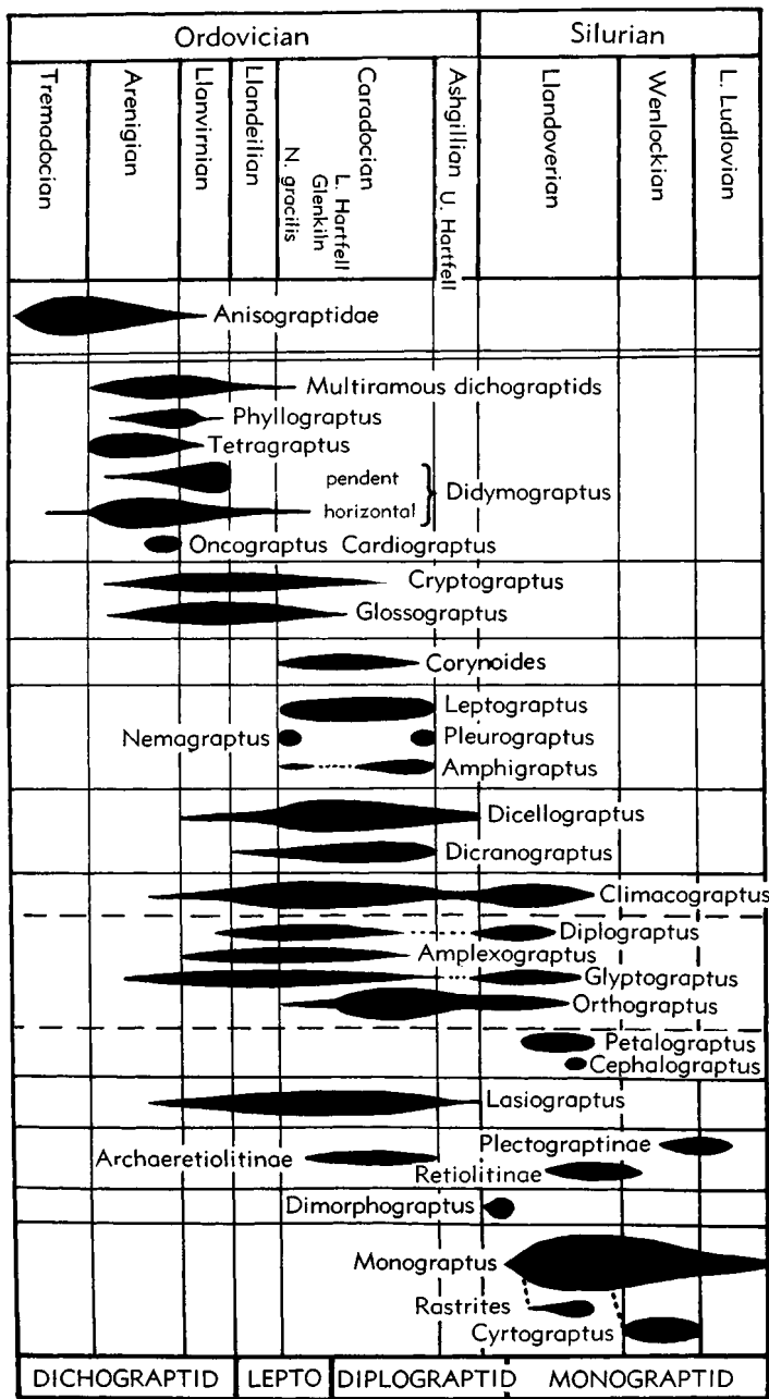
FIG. 5. Geological distribution of certain graptoloid genera. Number of species only approximately indicated; no attempt made to show relative importance of genera.
