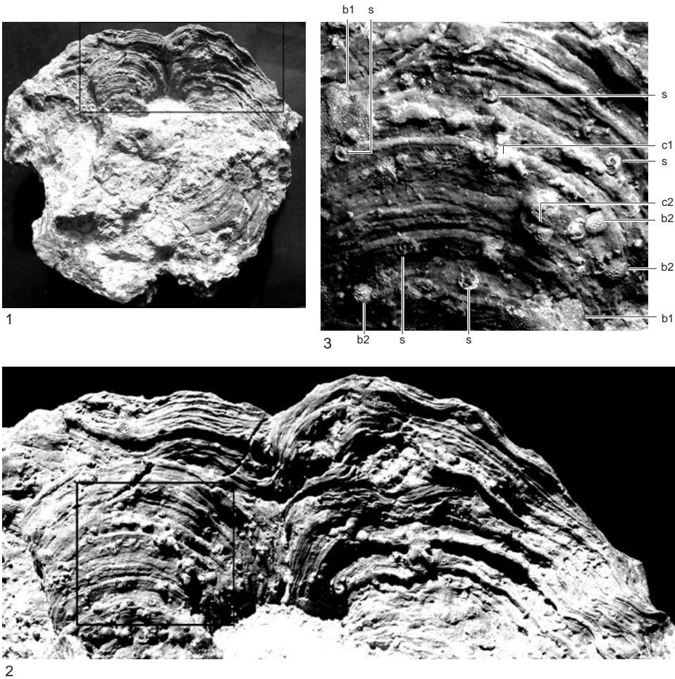
FIG. 310. Views at various magnifications of undersurface of a large, apparently coalescent, nonenveloping, low domical specimen of Parallelostroma sp., AMF.134350, Hamra Formation, Ludlow, Kättelviken, Gotland, Sweden. One area near margins of basal surface is well exposed and shows much detail of nature of corrugated base with growth rings and an abundance of cryptic encrusters (see views 2 and 3); upper surface is undulose and encrusted by a variety of organisms, including small, solitary rugosans and auloporoid corals; 1, general view of entire base of stromatoporoid Parallelostroma sp.; note the area outlined in black exhibits best-exposed part of basal surface (for more detail, see view 2), \times 0.25 (Webby & Kershaw, 2011); 2, corrugated basal surface of part of skeleton of stromatoporoid Parallelostroma sp.; note the two convex-outward sets of concentric growth ridges and an intervening zone with a locally sinuous, concave-outward, as well as upwardly steplike trend of growth ridges that seems to have formed in response to coalescing growth of specimen; in outer part of zone, growth ridges have continuity through sinuous and steplike changes of direction—steplike rise is from right to left; basal growth ridges appear to equate with distal ends of successive latilaminae (and/or laminae) within skeleton; a large number of cryptic encrusters are scattered over corrugated basal surfaces; box shows location of part illustrated in view 3, \times 0.85 (Webby & Kershaw, 2011); 3, enlargement depicting some of randomly distributed cryptic encrusters on corrugated underside of Parallelostroma sp. skeleton; they are completely randomly distributed over the corrugated basal surface; they did not preferentially occupy narrow groove-like hollows (potentially small primary occupation sites; see Fig. 305.6, inset) between individual growth ridges. Consequently, it is likely that these encrusters were predominantly colonizers of a large secondary shelter (overhang or cavity); b1 , sheetlike bryozoan; b2 , button-shaped bryozoan; c1 , crinoid with articulated plates; c2 , crinoid holdfast partly overgrown by bryozoan; s , Spirorbis , \times 1.8 (Webby & Kershaw, 2011).
