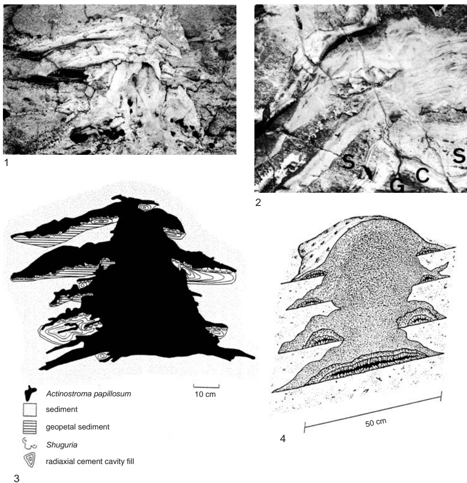
FIG. 292. Large, complex, free-standing, domical stromatoporoid that developed unsupported lateral outriggers off an elevated skeleton and was also colonized by cryptic organisms; these encrusted the sheltered sites beneath the extended outriggers, and the primary spaces were subsequently infilled by a combination of geopetal sediments and early marine cements. However, WOOD (2000, p. 678) inferred that at any one time during growth, the overall relief above the substrate would rarely be more than about one-third the total height of skeleton. The stromatoporoid adopting this growth form is Actinostroma papillosum BARGATZSKY, Frasnian, Upper Devonian, Pillara Limestone, Windjana Gorge, Canning Basin, Western Australia (see also Fig. 304; adapted from Wood, 1999, fig. CS 3.5b, copyright John Sibbick); 1, a large domical specimen of A. papillosum BARGATZSKY, \times 0.05 (Wood, 2000, fig. 6A); 2, part of a skeleton showing lateral outriggers of A. papillosum BARGATZSKY with lower surfaces encrusted by Shuguria (S), and cavities filled with sedimentary rock that form geopetal structures (G), and fibrous cement (C), \times 0.2 (Wood, 2000, fig. 6B); 3, outline drawn from the same large domical specimen (see view 1) to illustrate the nature of attached cryptic growth of Shuguria and cavities beneath lateral outgrowths containing geopetal structures and early marine cement (Wood, 2000, fig. 7A); 4, schematic drawing depicting inferred mode of growth of large domical stromatoporoid, with its important role in generating cryptobiont-bearing cavity spaces (Wood, 2000, fig. 6C; drawing courtesy of John Sibbick).
