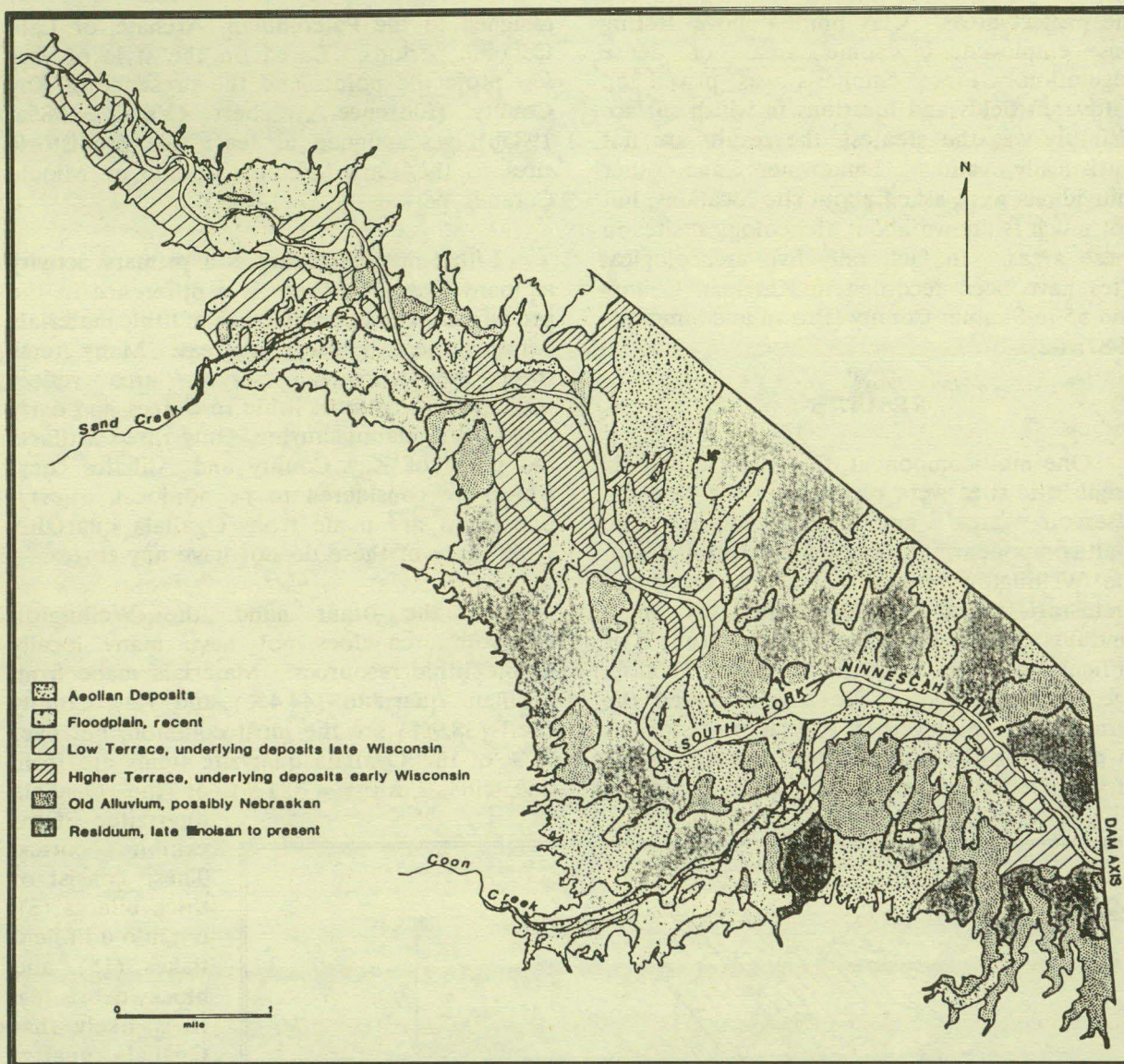
Figure 3. Soil groups within the Norwich reservoir.
