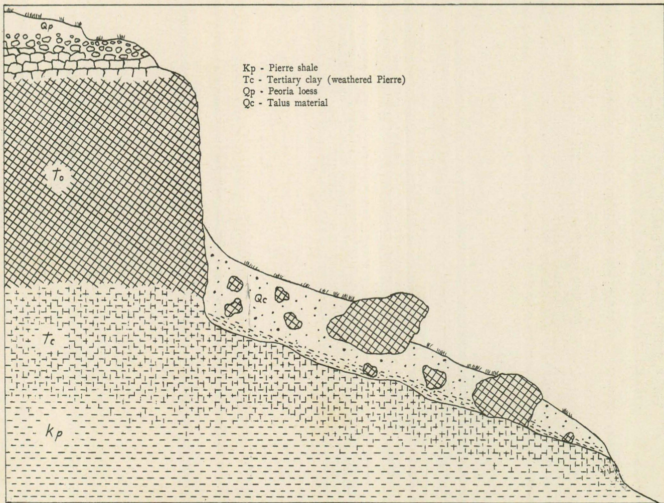
Figure 2. Generalized geologic section, vicinity of 14L01. No scale.
