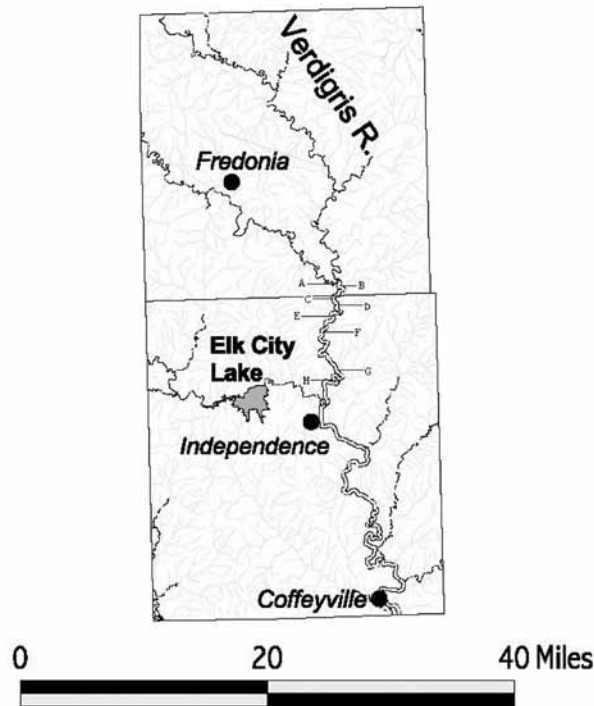
Figure 30. Map of the Verdigris River with sample sites (A-H) near the Eastep site, surveyed for live mussels in 2009–2010.
