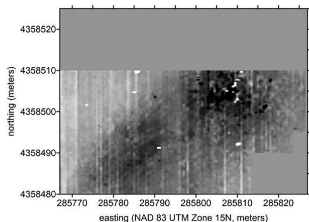
Figure 11. Magnetic susceptibility survey results.
