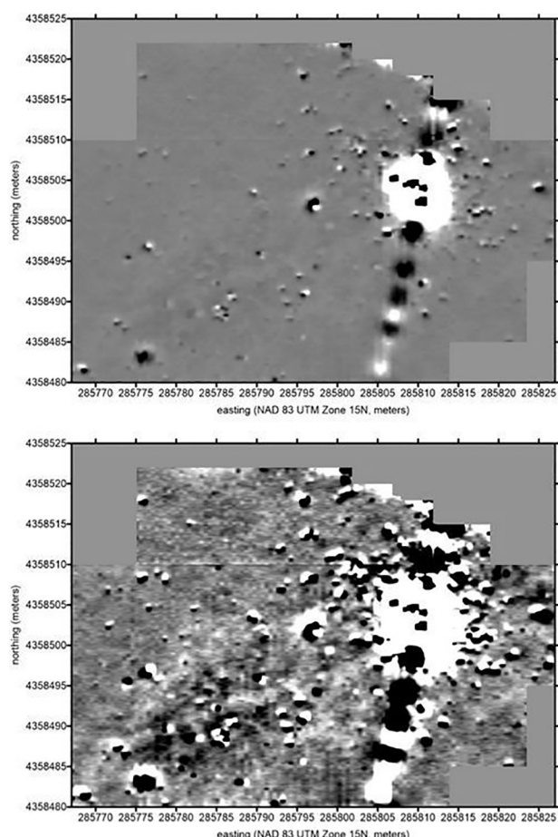
Figure 9. Magnetic field gradient survey results. Data presented at a contrast level of \pm 25 nT (above) and \pm 2 nT (below).
