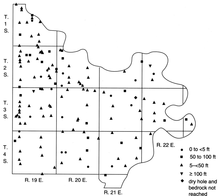
FIGURE 26—SATURATED THICKNESS OF PLEISTOCENE DEPOSITS, DONIPHAN COUNTY.
