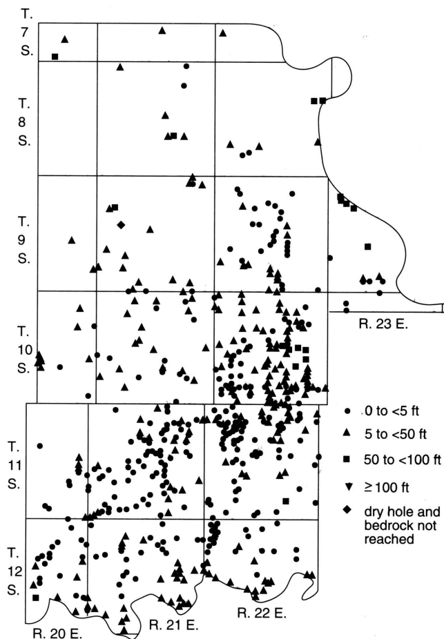
FIGURE 57—SATURATED THICKNESS OF PLEISTOCENE DEPOSITS, LEAVENWORTH COUNTY.
