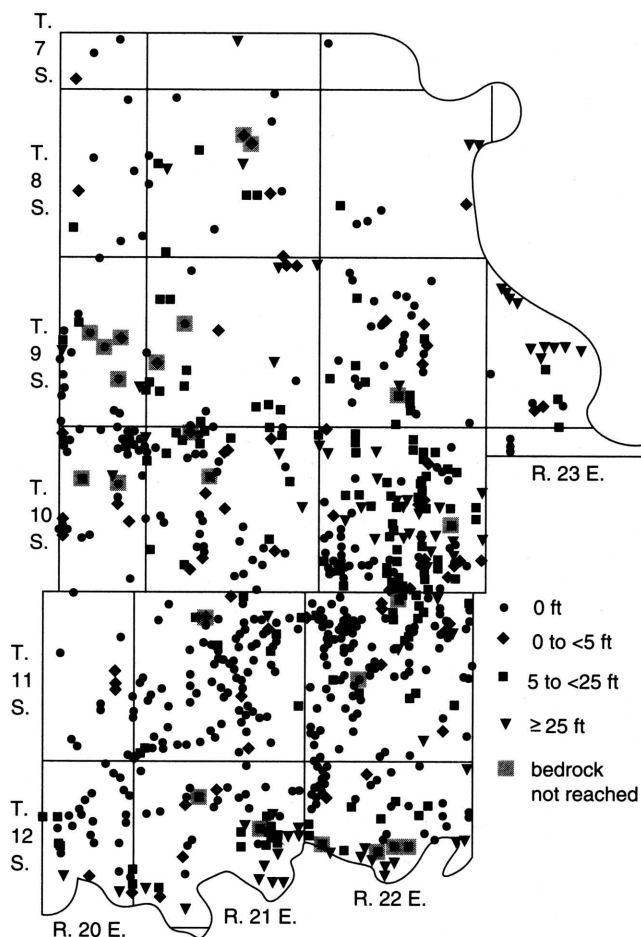
FIGURE 54—TOTAL PLEISTOCENE SAND AND GRAVEL THICKNESS, LEAVENWORTH COUNTY.
