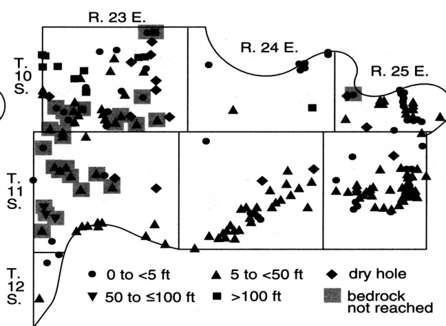
FIGURE 79—DEPTH TO WATER IN WELLS AND TEST WELLS, WYANDOTTE COUNTY.
