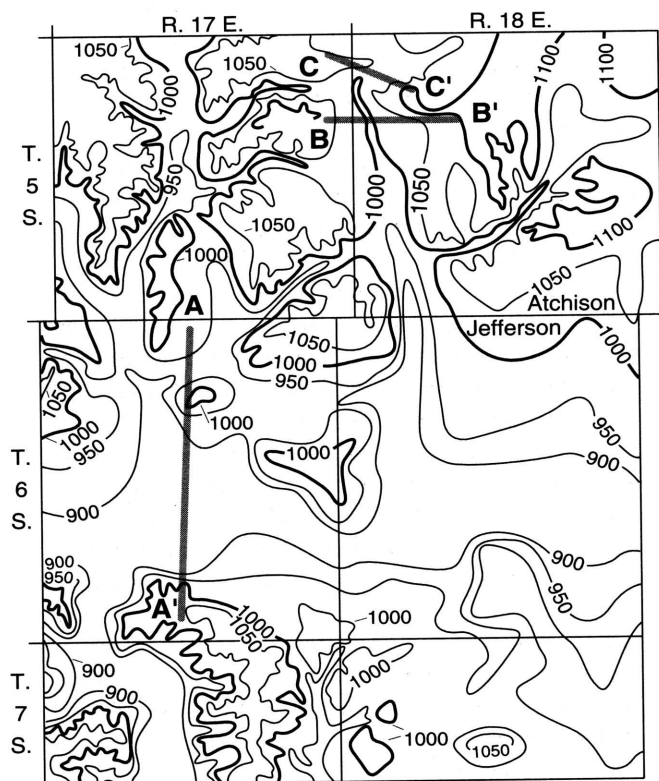
FIGURE 15—GEOLOGIC CROSS SECTIONS AND BEDROCK SURFACE IN WESTERN ATCHISON COUNTY.
