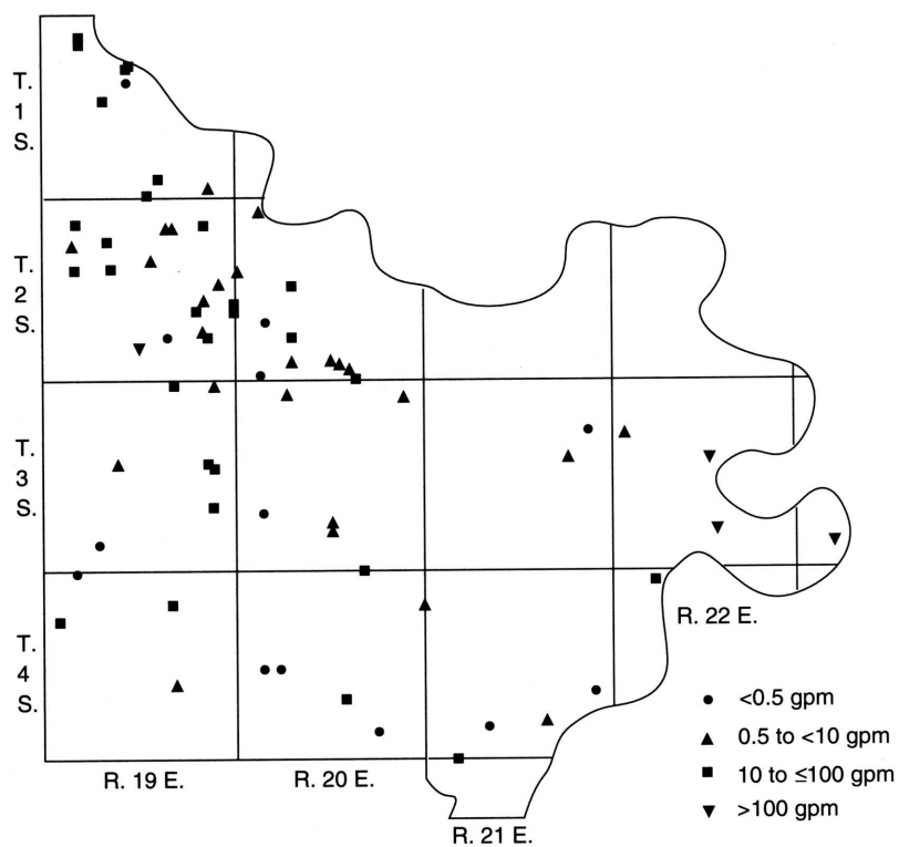
FIGURE 24—ESTIMATED WELL YIELDS, DONIPHAN COUNTY.
