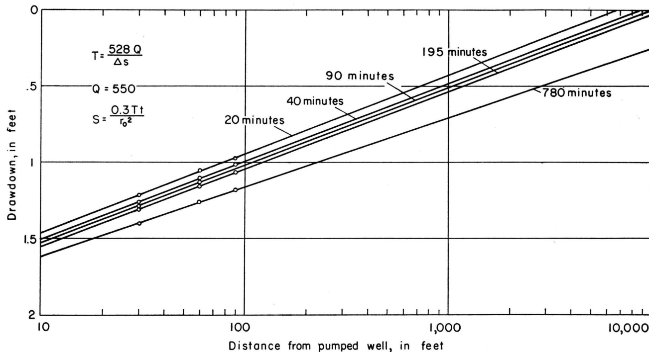
FIG. 10.—Drawdown of water level in observation wells 1E, 2E, and 3E at 20, 40, 90, 195, and 780 minutes plotted against distance from pumped well 10-11-2ca in Smith aquifer test.
