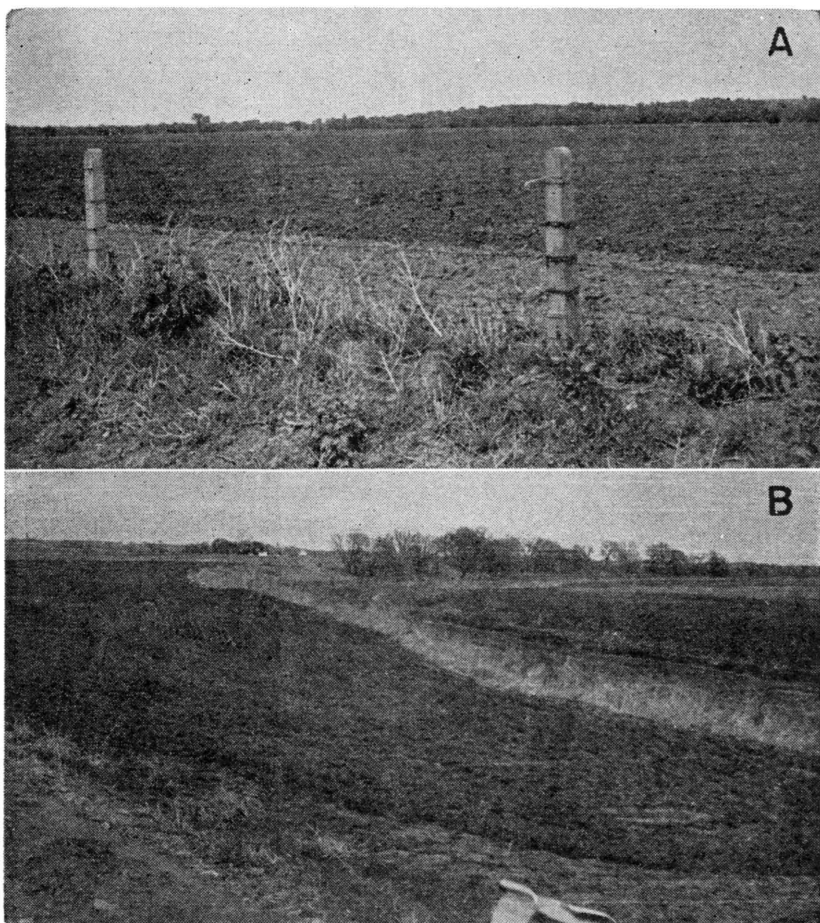
PLATE 8.—A, Newman Terrace surface in Mill Creek valley, looking northeast from a point about half a mile southeast of Maple Hill. B, Scarp between Newman Terrace and flood plain in SW \frac{1}{4} sec. 29, T. 10 S., R. 13 E.
