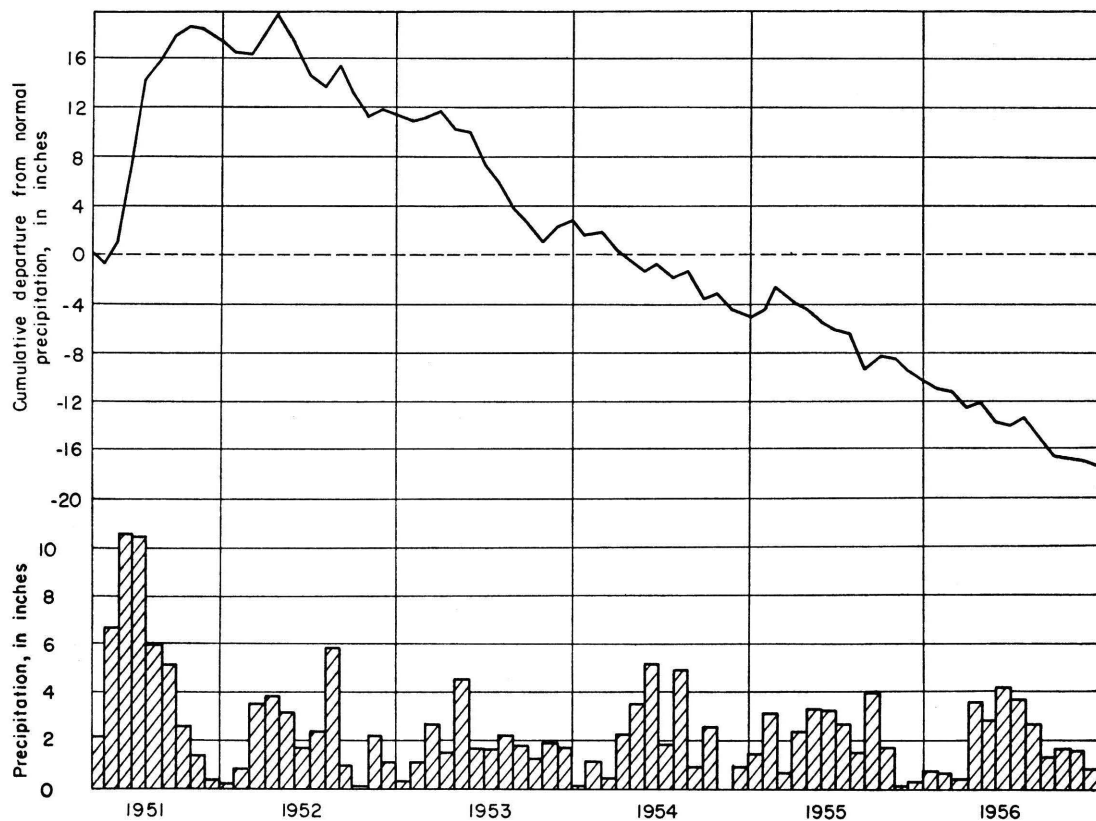
FIG. 3.—Monthly precipitation and cumulative departure from normal at Willard for the period April 1951 to January 1957.
