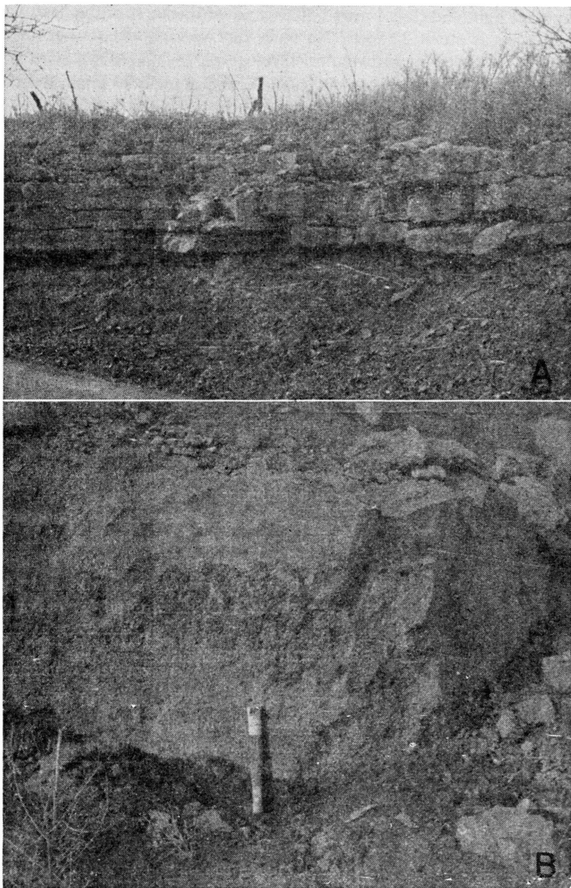
PLATE 4.—A, Silver Lake Shale and overlying Burlingame Limestone in road cut in SE \frac{1}{4} NE \frac{1}{4} sec. 36, T. 11 S., R. 14 E. B, Tarkio Limestone in quarry in sec. 29, T. 11 S., R. 14 E.
