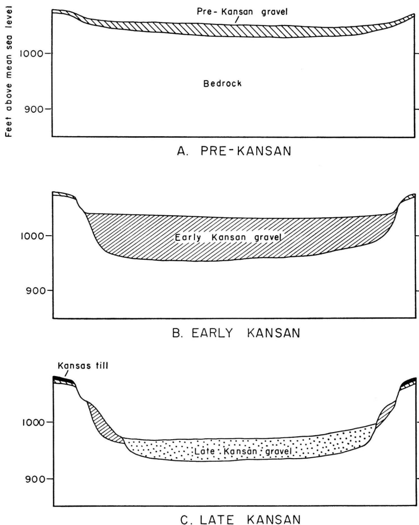
FIG. 4.—Idealized geologic sections showing development of Kansas River valley.
