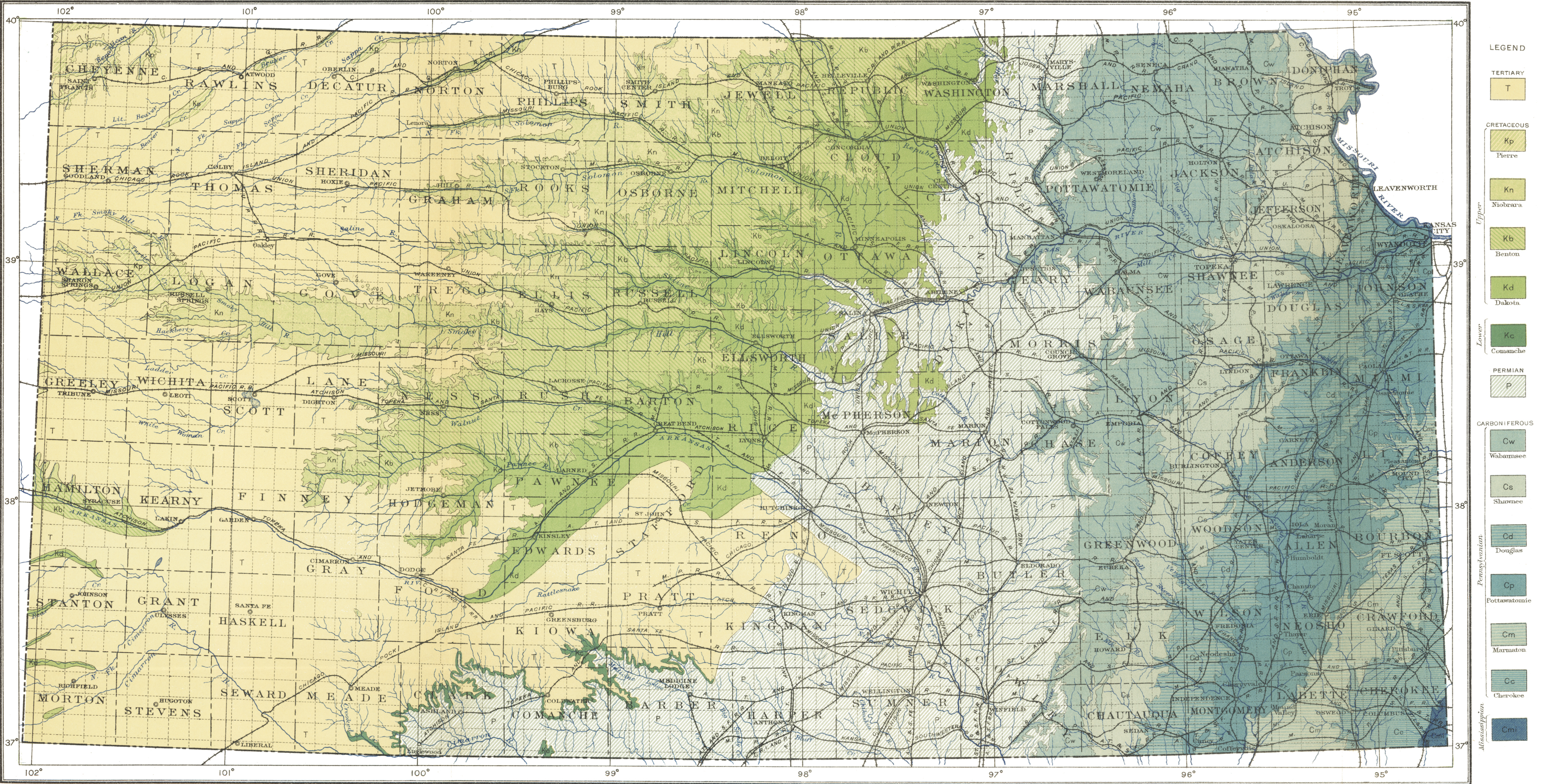
GEOLOGIC MAP OF KANSAS Prepared under the direction of Erasmus Haworth, State Geologist Scale: 1 inch = 24 miles 10 0 10 20 30 40 50 60 Miles 1913
