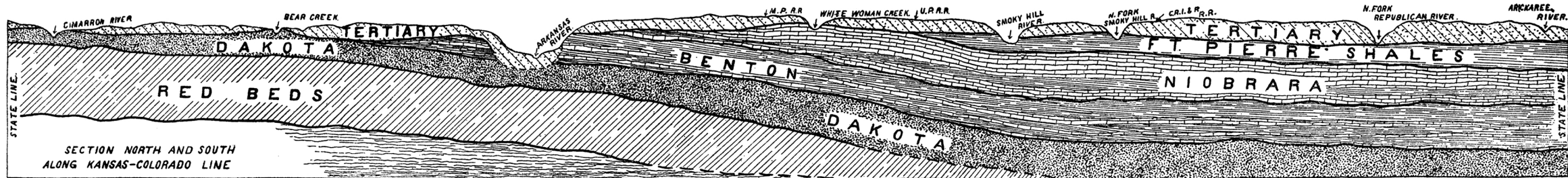
A geologic cross section from north to south along the west end of Kansas, showing relations of different formations to each other and to the water-bearing Tertiary.
