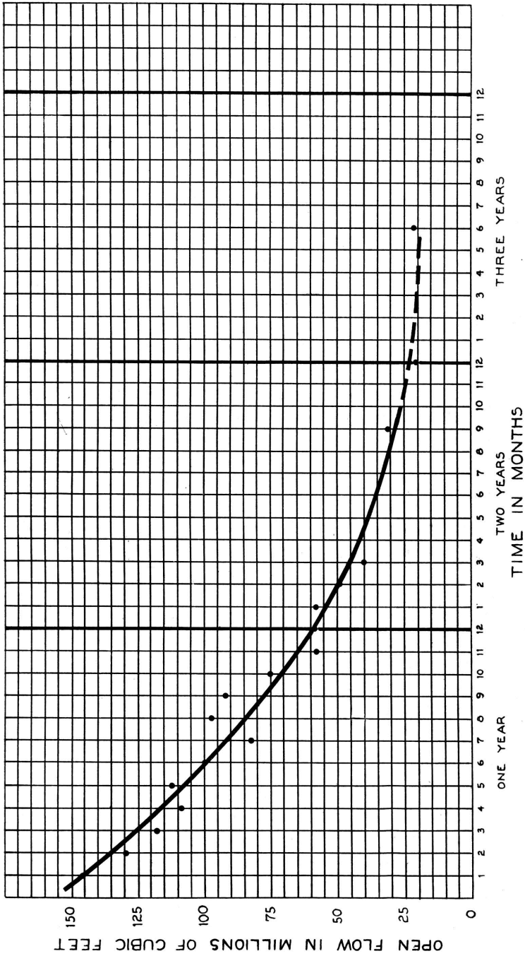
FIG. 8.—Open flow decline curve of the chief properties in the Polkinghorn gas field.
