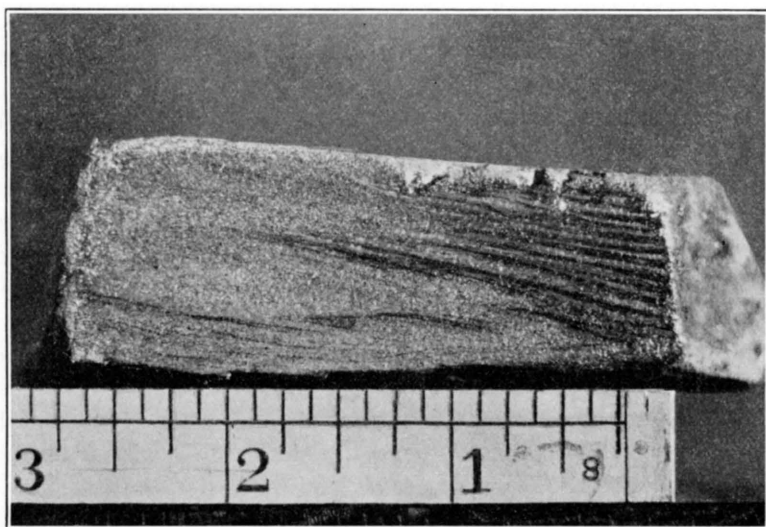
FIG. 12.—Fragment of sand from the Bush City shoestring. The fine cross-bedding is shown by dark streaks of silt and flakes of mica that line the irregular bedding planes which separate the cleaner bands of sand. This channel sand retains a large percentage of its oil because of its fineness and lenticular structure of impure material. ( Scale in inches. )
