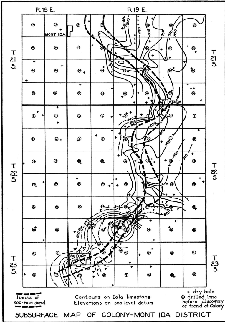
FIG. 9.—Subsurface structural map of the Colony-Mont Ida district.
