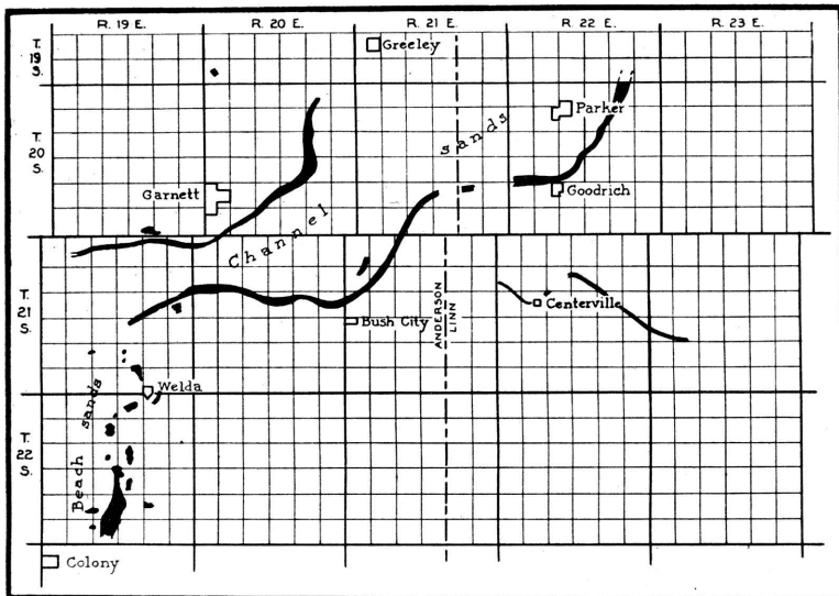
FIG. 5.—Deposits of the 800-foot, or “shoestring” sand, in the Anderson-Linn county district. The two types of sand bodies at the same horizon throw some light on the paleogeography of the time. It seems likely that other channels are in the area south of Bush City and Centerville. (Base map after Rich.)
