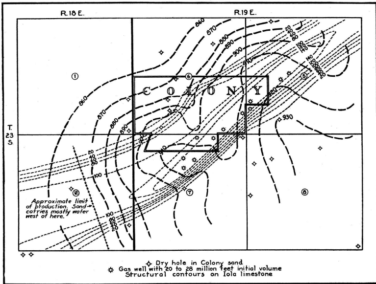
FIG. 11.—Sand-thickness and subsurface structural map of the Colony gas field. The isobaths, or sand-thickness contours, are assumed from data furnished by dry holes on the edges of the sand, from wells which penetrated 100 feet or more, and from a well in sec. 5 that was drilled through the sand where it was 135 feet thick. The oblong shape of the thickest portion is based on the arrangement of the wells of large initial volume. The position of the thin edges is too uncertain to be indicated.
