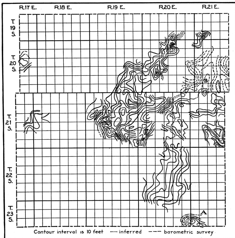
Fig. 2.—Surface structural map of Anderson county. The map demonstrates the unsystematic type of structure in the county. Contours are drawn on different limestone beds, chiefly the Iola and Plattsburg. A is believed to represent a structure caused by folding; B a structure caused by thinning of a shale member beneath the limestone used for datum. The map is a compilation of the work of several geologists and includes a large part of the area occupied by key beds. The regional dip is toward the northwest.
