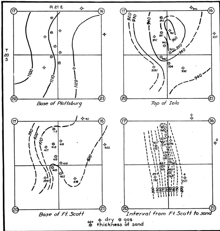
FIG. 3.—These plats indicate the unreliability of structural evidence in connection with small isolated sand deposits. Poorly recorded well logs, used in this instance without attempt for correction, account for some of the oddities of structure. The dip of the surface beds, as mapped on the base of the Plattsburg limestone, is practically normal, but the area shown is on the west flank of an anticline. If differential settling is the only cause of the flexure, the more pronounced dips should be in the Fort Scott limestone. The contours on the base of this member suggest that later westward tilting of the strata increased the "compaction-dip" above the down-dip flank of the sand body and decreased it above the up-dip flank. The plat at the lower right shows that the sand is a bar-shaped ridge with relief of at least 44 feet. The producers are confined to one row of wells along the crest.
