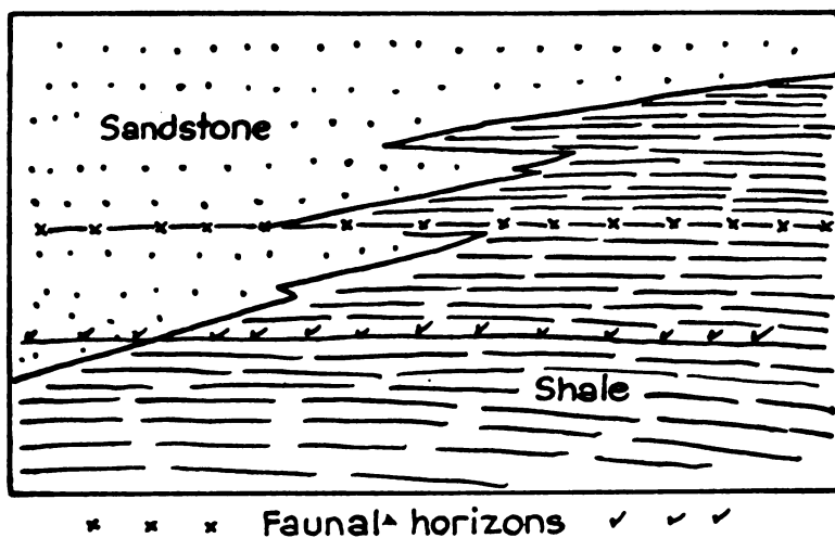
FIG. 5.—Diagram showing gradation of shale into sandstone, with faunal horizons persisting through both types of rock.
