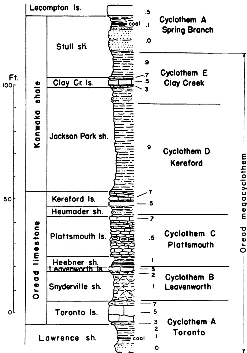
FIG. 3.—Diagram showing typical megacyclothem of the Shawnee group.
