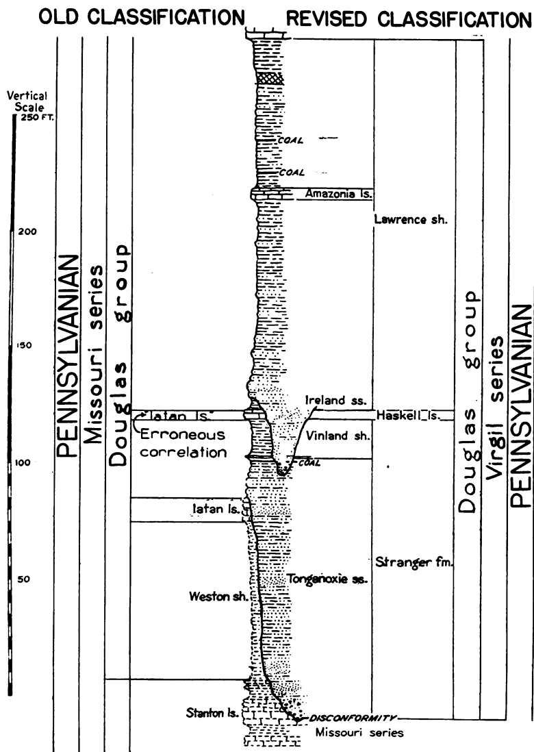
FIG. 9.—Diagram showing comparison of old and revised classification of lower Virgil beds. The unconformity that separates the Stranger formation from the Iatan, Weston, or Stanton beds was not recognized in earlier work.
