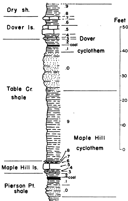
FIG. 2.—Diagram showing two typical cyclothem in the Wabaunsee group. The relation of formational stratigraphic divisions to the cyclothem is also indicated.
