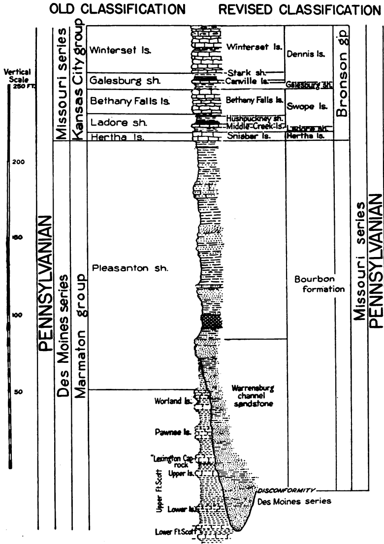
FIG. 7.—Diagram showing comparison of old and revised classification of lower Missouri beds (redefined).
