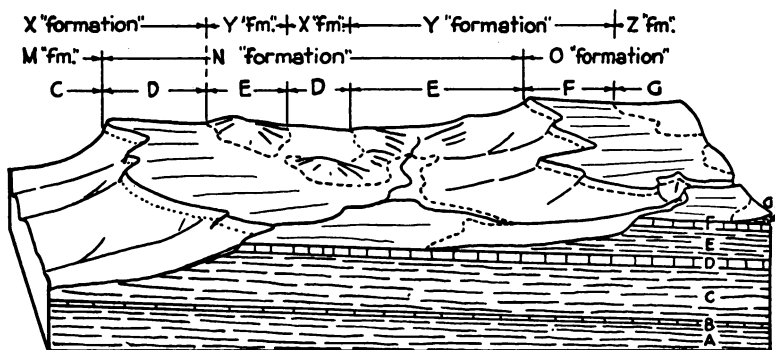
FIG. 1.—Generalized diagram of formation boundaries. A to G, limestone and shale members. M to O, formations defined from base of one hard member to next. X to Z, formations defined from top of one hard member to next. Clearly, the boundaries between units C and D, E and F, are the most readily mapped.
