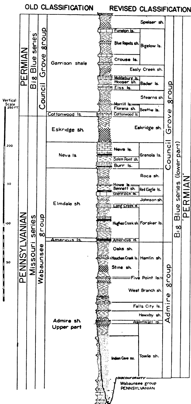
FIG. 12.—Diagram showing comparison of old and revised classification of beds now referred to the lower part of the Big Blue series of "Permian" age. This shows especially the revision of the boundary between the Pennsylvanian and "Permian" rocks.
