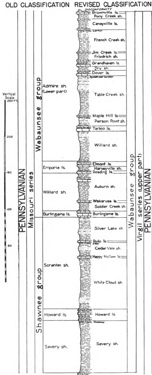
FIG. 11.—Diagram showing comparison of old and revised classification of upper Virgil beds.
