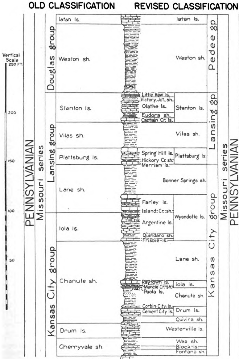
FIG. 8.—Diagram showing comparison of old and revised classification of upper Missouri beds (redefined).
