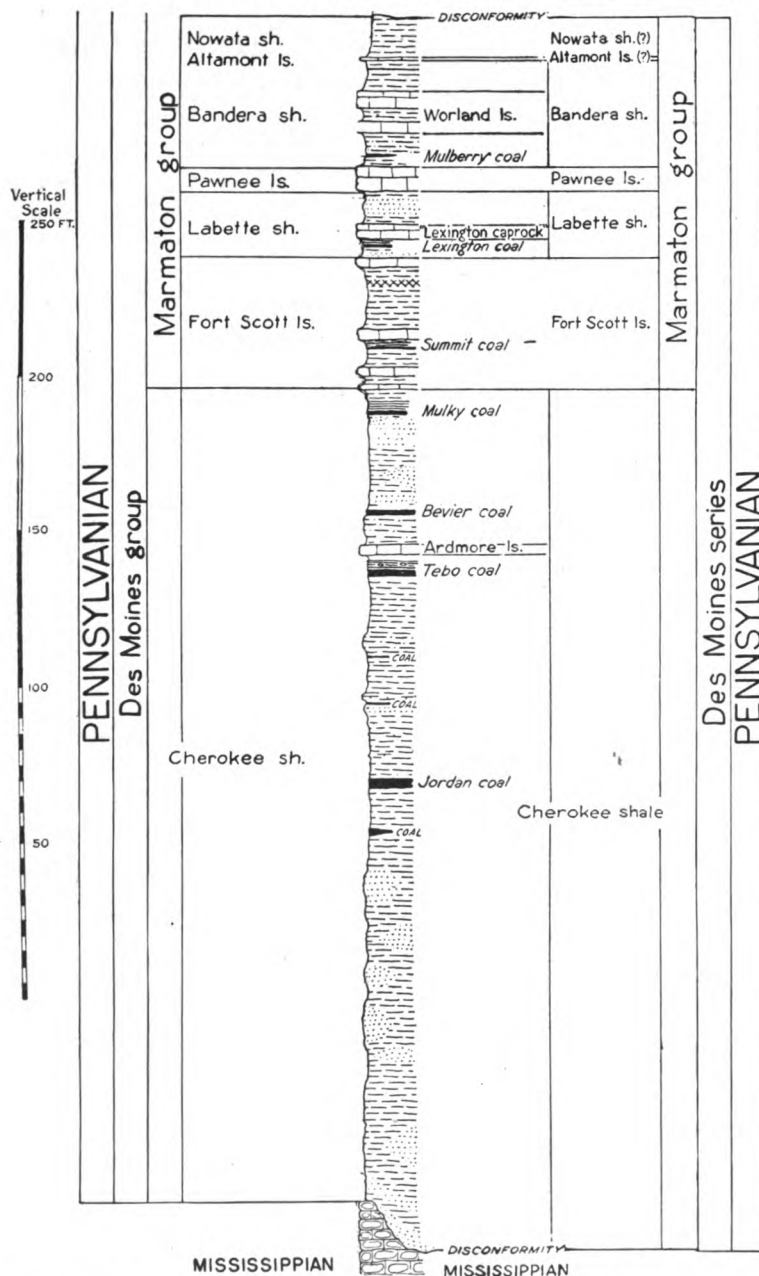
FIG. 6.—Diagram showing comparison of old and revised classification of Des Moines beds. This section, representing conditions in the latitude of the Kansas river, does not show the most typical development of the Marmaton beds. In southeastern Kansas the Lenapah limestone appears above the Altamont and beneath the disconformity that marks the base of the Missouri series, as redefined.
