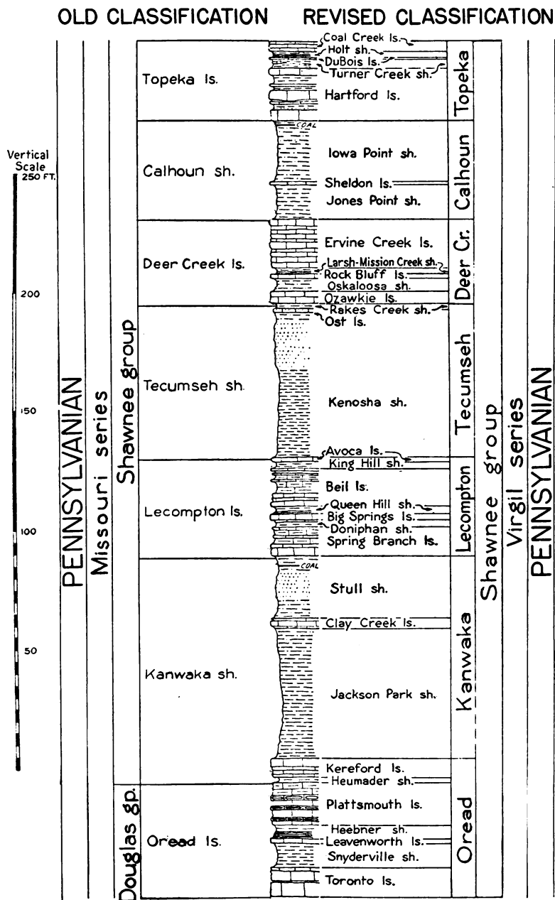
FIG. 10.—Diagram showing comparison of old and revised classification of middle Virgil beds.
