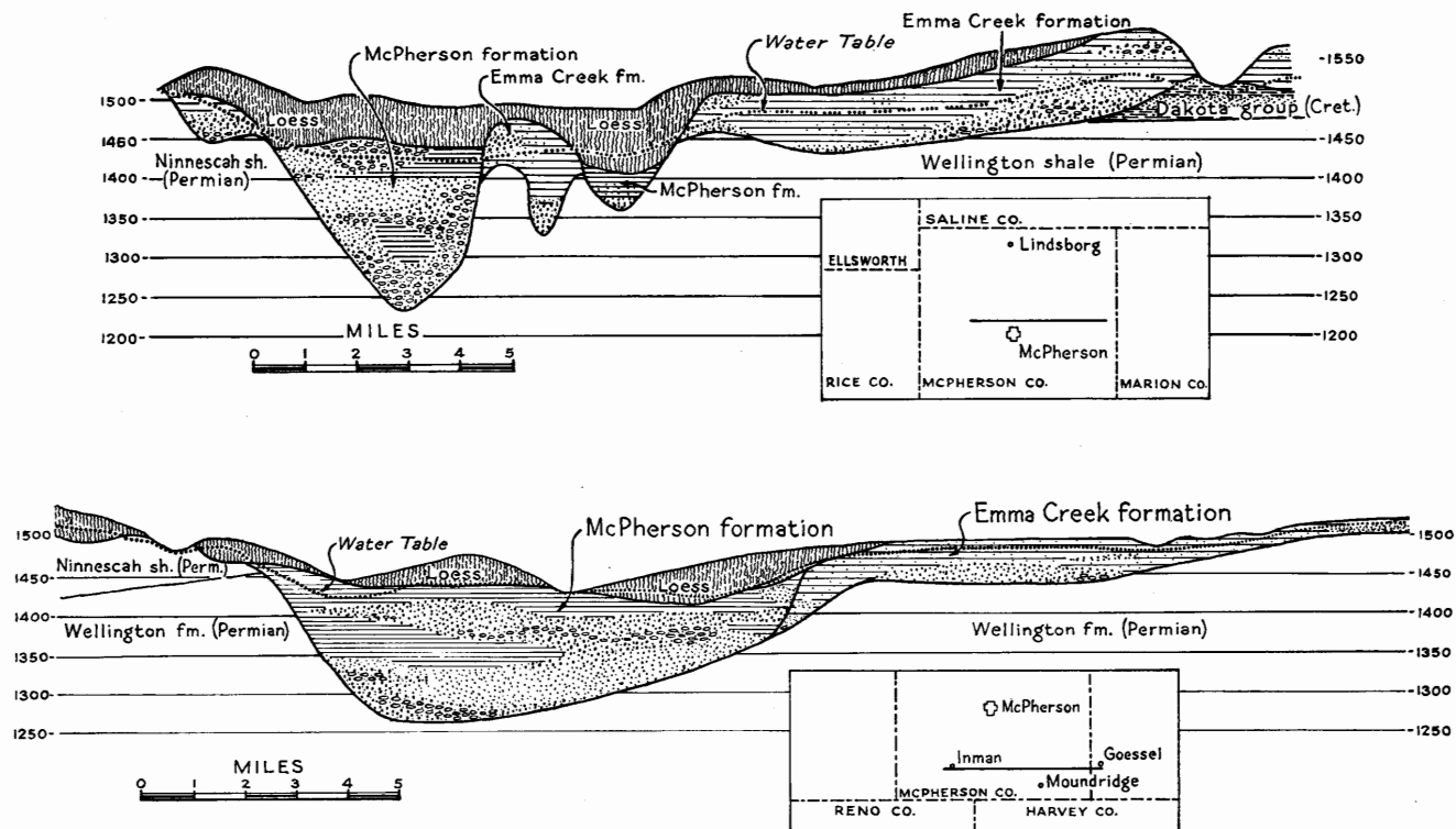
FIG. 25. Geologic sections of water-bearing alluvial deposits belonging to the Emma Creek (Tertiary) and McPherson (Quaternary) formations in McPherson county. Very large quantities of good ground water are obtainable from the McPherson deposits. (J. C. Frye.)
