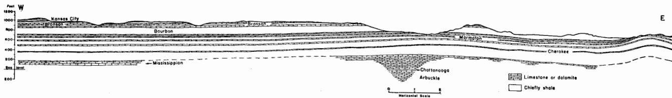
FIG. 21. Geologic section in an east-west direction across central Linn county. Limestone beds that occur next below the land surface over many square miles are good sources of ground-water supply. The water is collected in openings dissolved along bedding planes and joint cracks and it tends to migrate slowly in the direction of dip of the beds. (J. M. Jewett.)
