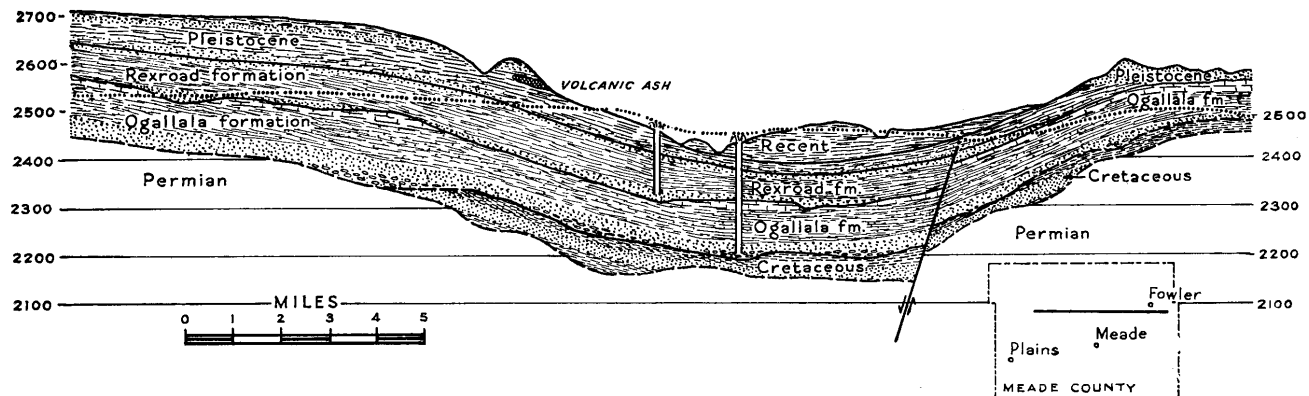
FIG. 27. Geologic section of a portion of the Meade artesian basin, Meade county. Structural conditions that are responsible for the local artesian flow of wells are represented. The pre-Tertiary and Ogallala rocks are displaced by a fault that is observed to mark the local boundary of distribution of certain Pleistocene deposits (lower and middle Rexroad beds), which indicates that the displacement is mostly pre-Pleistocene in date. The thickness of Cretaceous rocks and the structure of the pre-Tertiary rocks are interpreted from studies in adjacent areas; they are not based on information from wells in this region. (J. C. Frye.)
