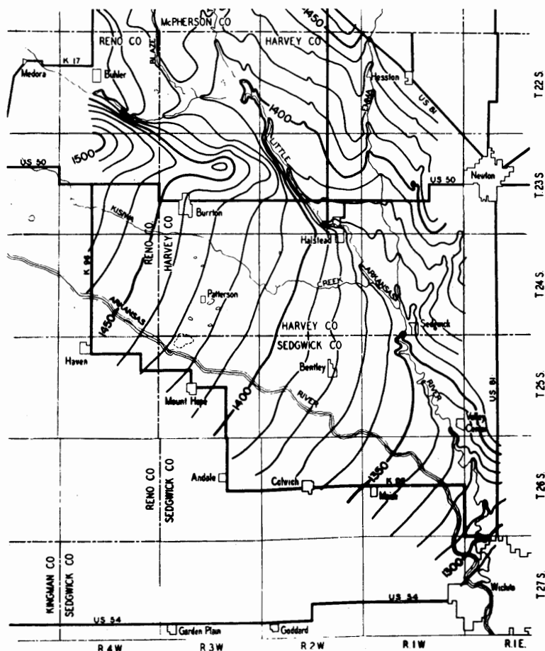
FIG. 26. Map of the ground-water table in an area surrounding Halstead, Kan. The progressively lower elevation of the table from northwest to south-east indicates that the general direction of ground-water movement is south-eastward. The relatively high position of the table adjacent to the sand-hills area northeast of Hutchinson reflects the influence of favorable recharge conditions in the sand area.
