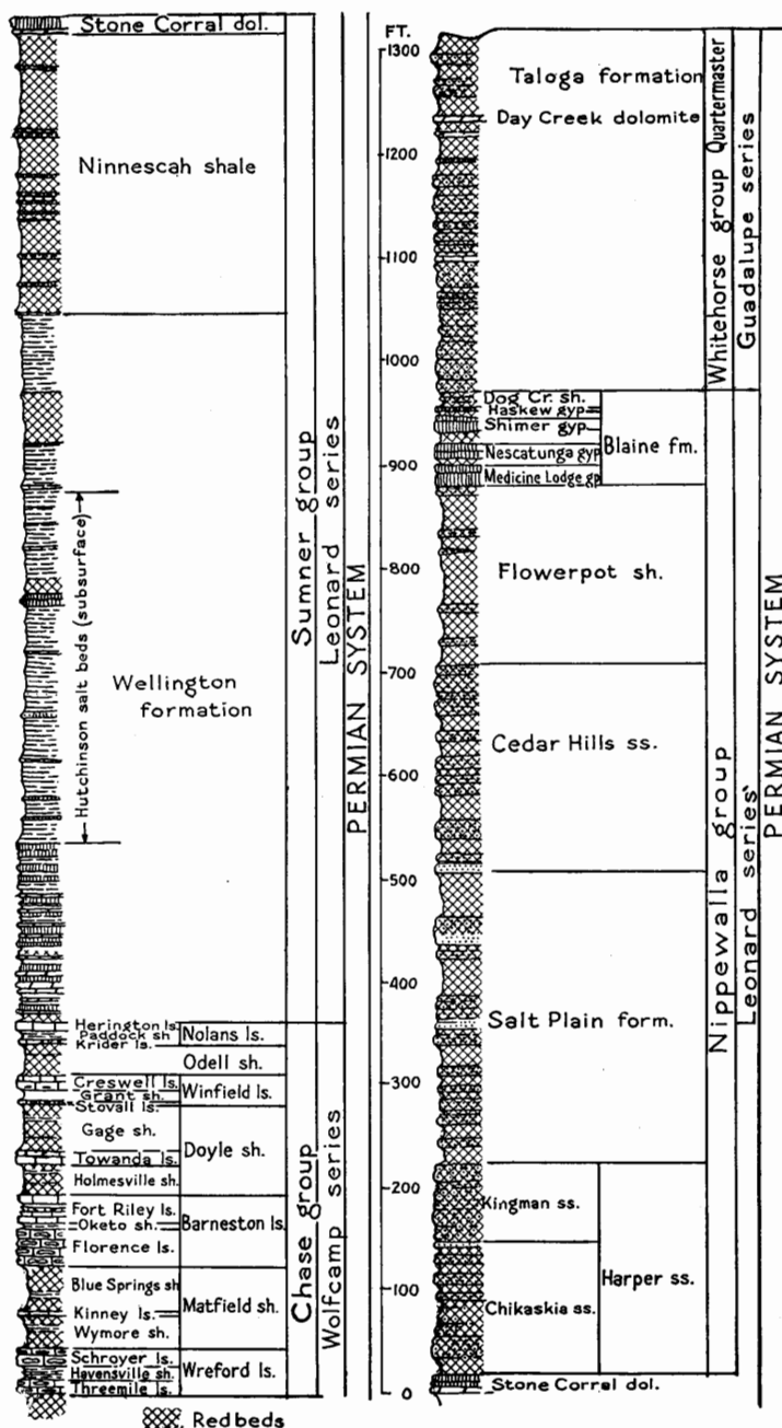
FIG. 15. Generalized section of the middle and upper parts of the Permian system in Kansas, based mainly on outcrops in south-central counties. Wide-spread salt deposits in the middle part of the Wellington formation are not indicated in the section because the salt is penetrated only in deep wells. Ground-water supplies in these rocks are scanty and poor.
