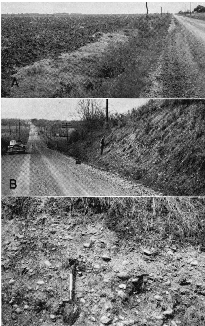
PLATE 8.—A, Part of extensive plain in Hesper area developed on Kansan glaciofluvial deposits. View south from near center W. side NE \frac{1}{4} sec. 27, T. 13 S., R. 21 E.; B, Toe of Menoken Terrace along north side of Kansas River valley, S. side SW \frac{1}{4} sec. 9, T. 12 S., R. 20 E. Terrace-shale contact about at position of automobile. Newman Terrace surface in background; C, Poorly sorted Grand Island gravel and sand in basal Menoken Terrace deposits exposed just right of center in 8B.
