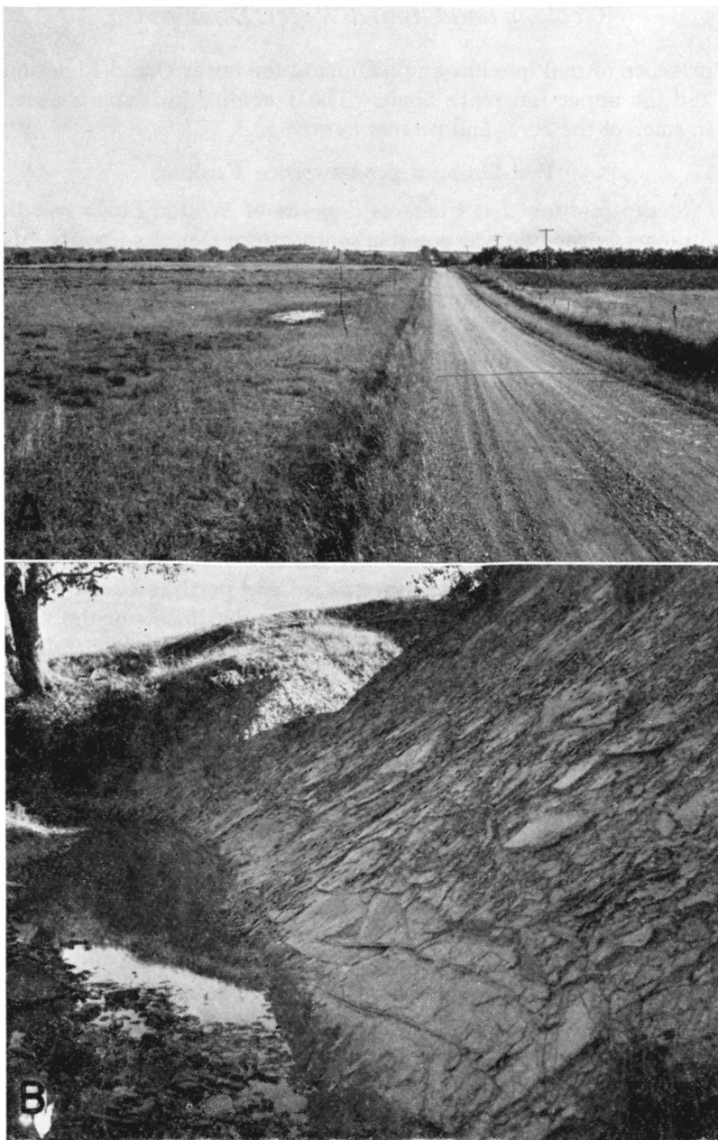
PLATE 9.—A, Nearly circular small water-filled sinkhole developed in Plattsmouth Limestone member of the Oread Limestone along Worden fault in the SE \frac{1}{4} NW \frac{1}{4} sec. 33, T. 14 S., R. 19 E., Plattsmouth member underlies surface in foreground and also hill 40 feet higher in background; B, Shale beds dipping 35° E. in post-Stranger pre-Ireland fault block adjacent to channel containing Ireland Sandstone member of Lawrence Shale. Normal dip of beds in this area is less than \frac{1}{2} ° NW. Tilted shale beds overlain by undisturbed beds of Ireland member. View south from NE cor. SW \frac{1}{4} sec. 33, T. 14 S., R. 21 E.
