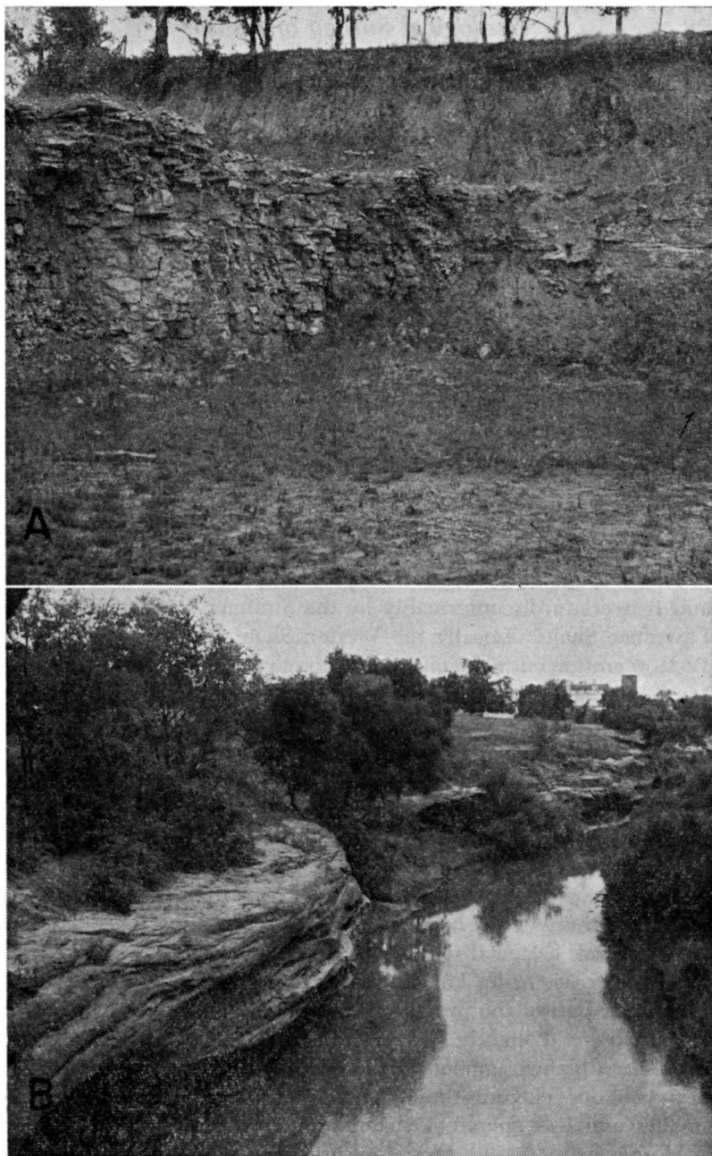
PLATE 4.—A, Stoner Limestone member of Stanton Limestone overlain by Kansan glaciofluvial deposits in quarry, NE cor. sec. 4, T. 13 S., R. 21 E.; B, Massive Tonganoxie Sandstone member of Stranger Formation at Dightman's Crossing, Wakarusa River, NE \frac{1}{4} NE \frac{1}{4} sec. 14, T. 13 S., R. 20 E.
