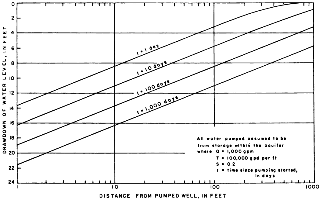
FIGURE 6.—Drawdown of water level at any distance from the pumped well after pumping has begun.
