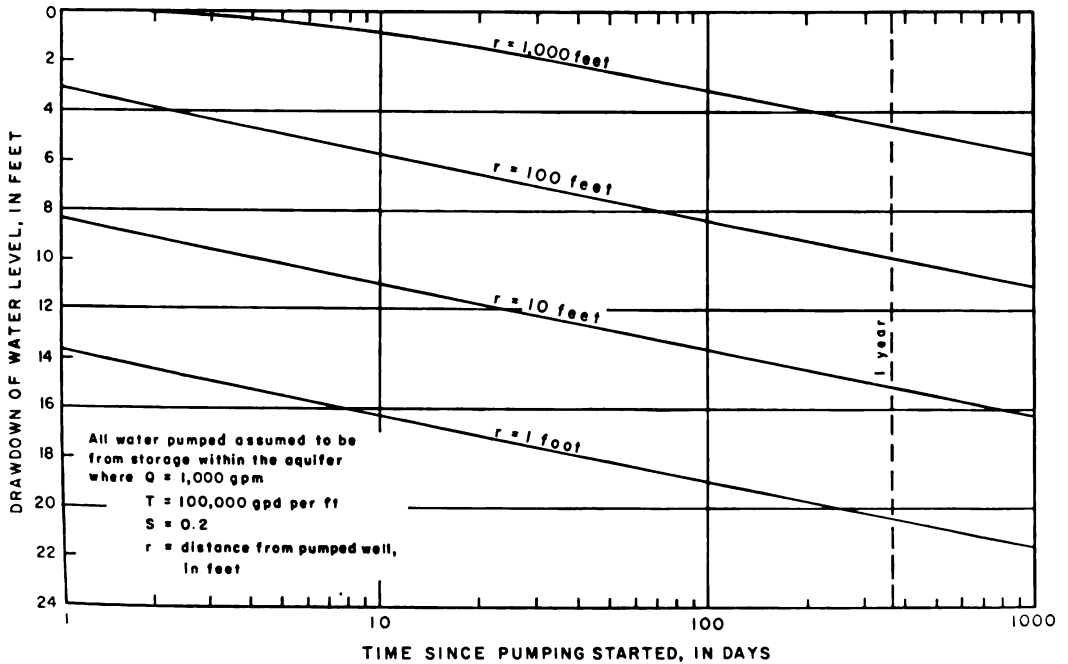
FIGURE 7.—Drawdown of water level at any time after pumping has begun.
