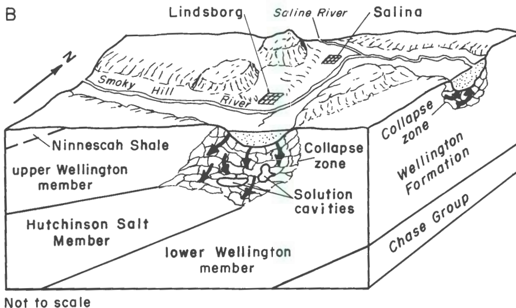
Figure 4.--Conceptual block diagrams near Lindsborg showing geologic development, mechanism of dissolution of the Hutchinson Salt Member, and development of Wellington aquifer between Cretaceous time (A) and present (B).
