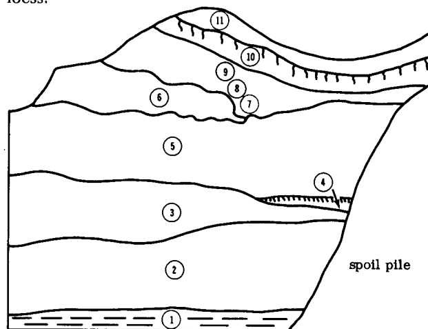
WATHENA SOUTH #2 SECTION
