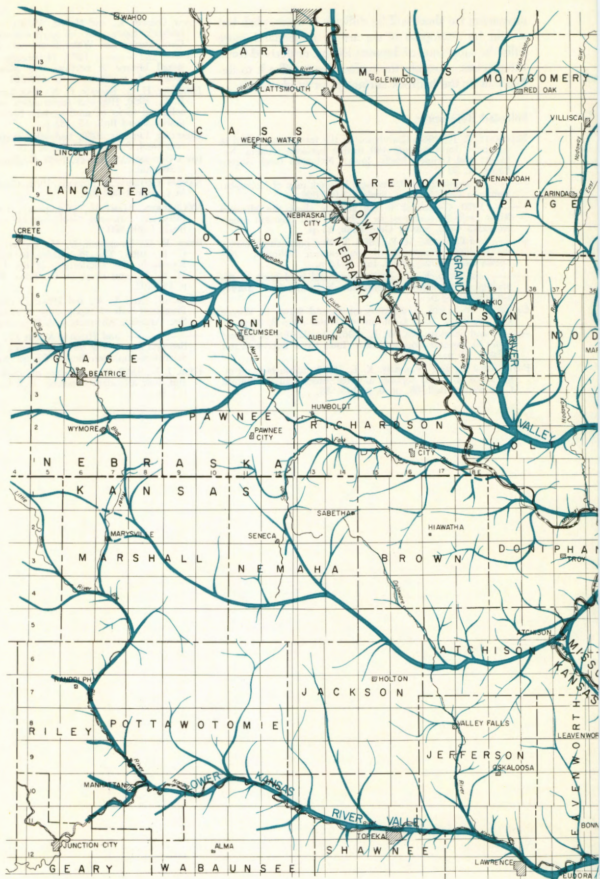
FIGURE 1.—Preglacial drainage map of the lower Missouri Basin.
