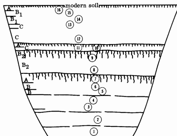
NEWTON FARM SECTION
