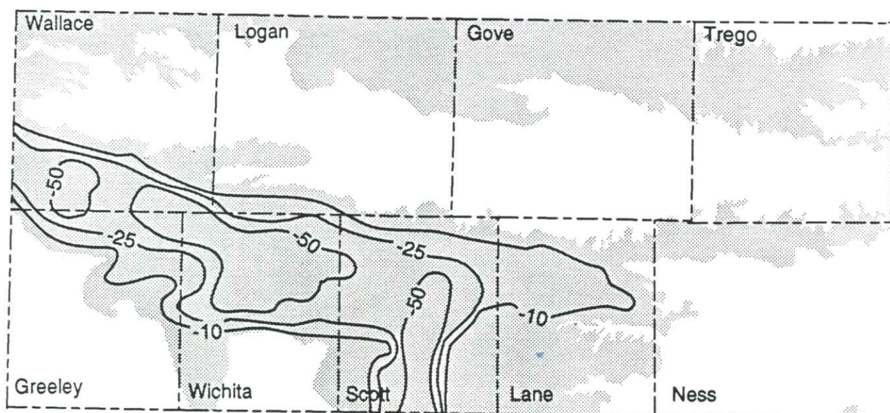
FIGURE 10C—MAP OF THE ANNUAL CHANGE IN WATER LEVEL IN REGION II, WEST-CENTRAL KANSAS, SINCE THE LAST REPORT. Values of the contours are the observed changes in water level in feet.
