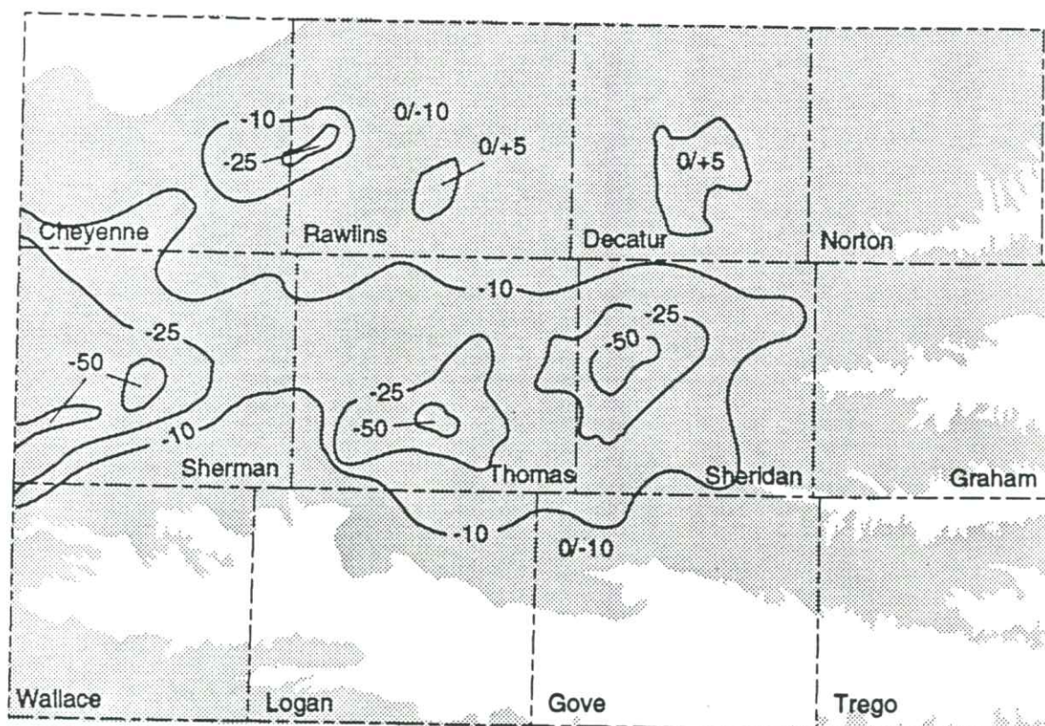
FIGURE 11B—MAP OF PERCENT CHANGE IN PREDEVELOPMENT SATURATED THICKNESS FOR REGION III, NORTHWEST KANSAS.
