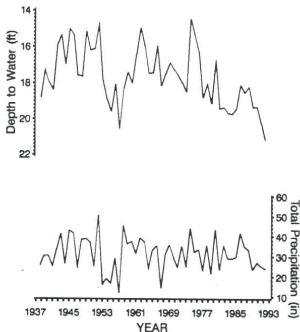
FIGURE 7—COMPARISON OF PRECIPITATION WITH WATER LEVEL IN SEDGWICK COUNTY WELL, 25S01W26DBD01 [Pleistocene alluvial formation]. Precipitation records are from the Sedgwick station.
