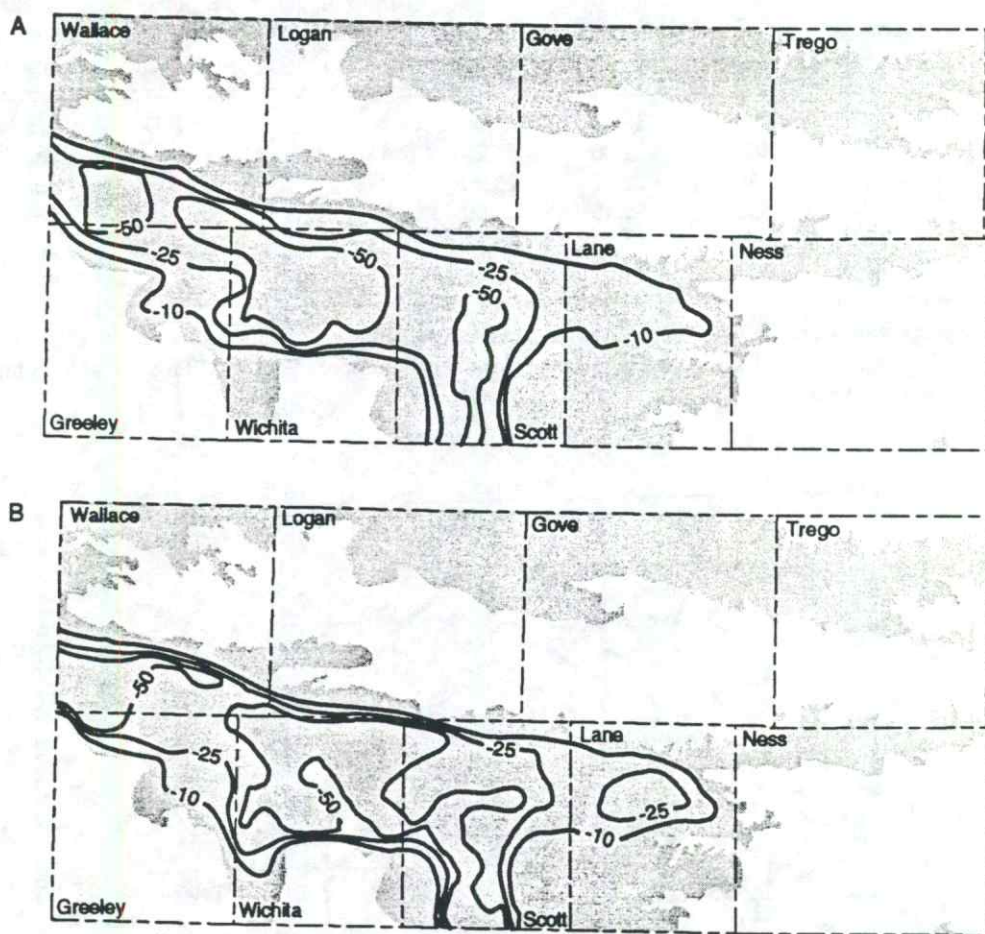
Figure 10. (A) Generalized water-level change (in feet) in region II, west-central Kansas, predevelopment to 1993. (B) Change (%) in saturated thickness in region II, west-central Kansas, predevelopment to 1993. (C, opposite ) Annual water-level change (in feet) in region II, west-central Kansas, for 1993.
