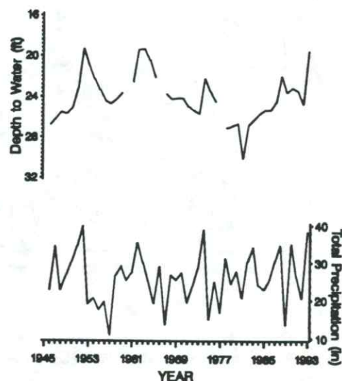
Figure 5. Comparison of precipitation at Cawker City (station 14137102) with water levels in Osborne County well 06S 12W 23 CDC 01 [30 ft (9.1 m) deep, alluvial formation].
