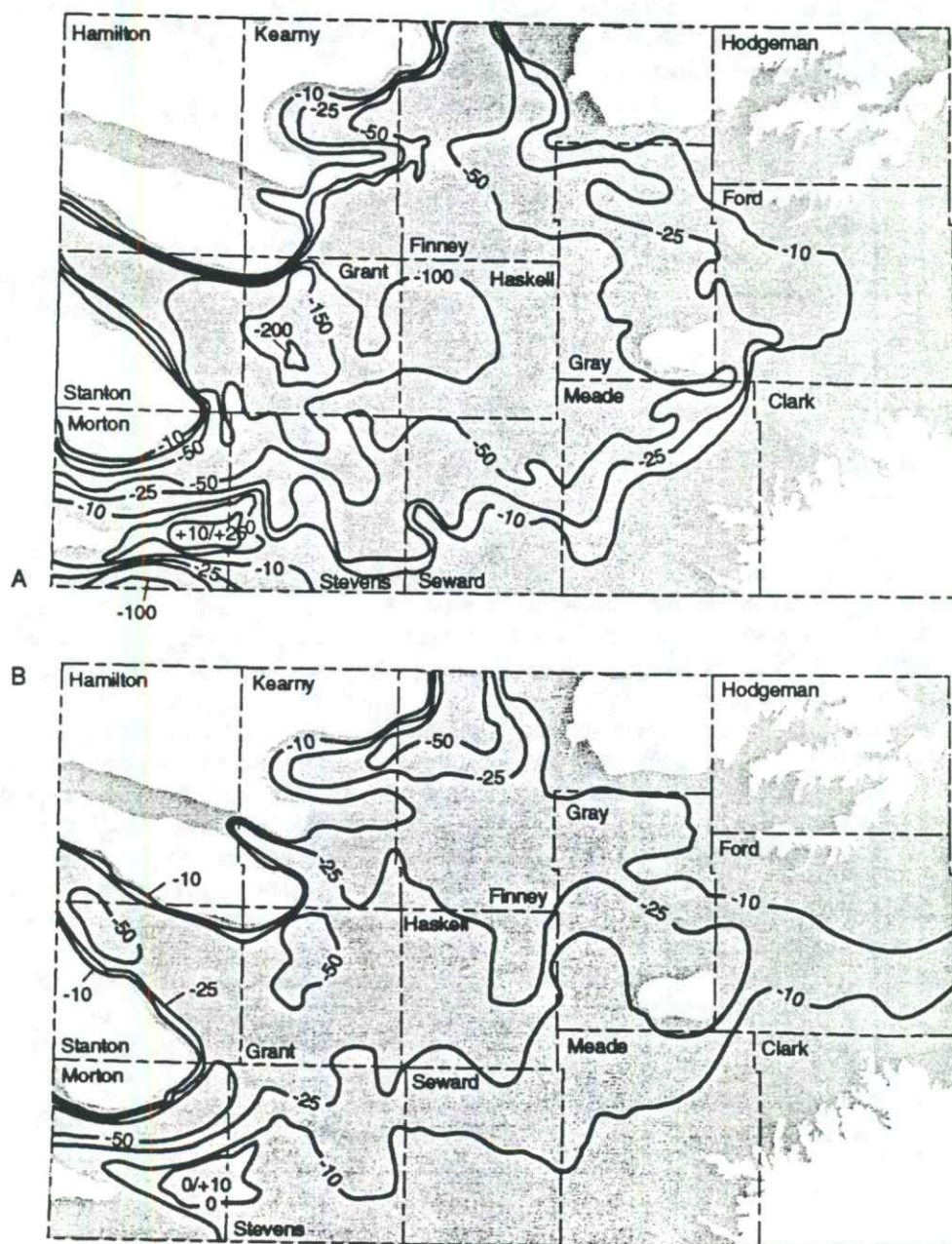
Figure 9. (A) Generalized water-level change (in feet) in region I, southwest Kansas, predevelopment to 1993. (B) Change (%) in saturated thickness in region I, southwest Kansas, predevelopment to 1993. (C, opposite) Annual water-level change (in feet) in region I, southwest Kansas, for 1993.
