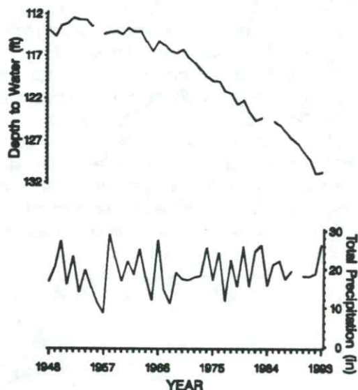
Figure 8. Water levels in Thomas County well 08S 34W 01 BAC 01 [160 ft (48.8 m) deep, Ogallala Formation]. Compared with precipitation at Colby 1 SW (station 14169901).
