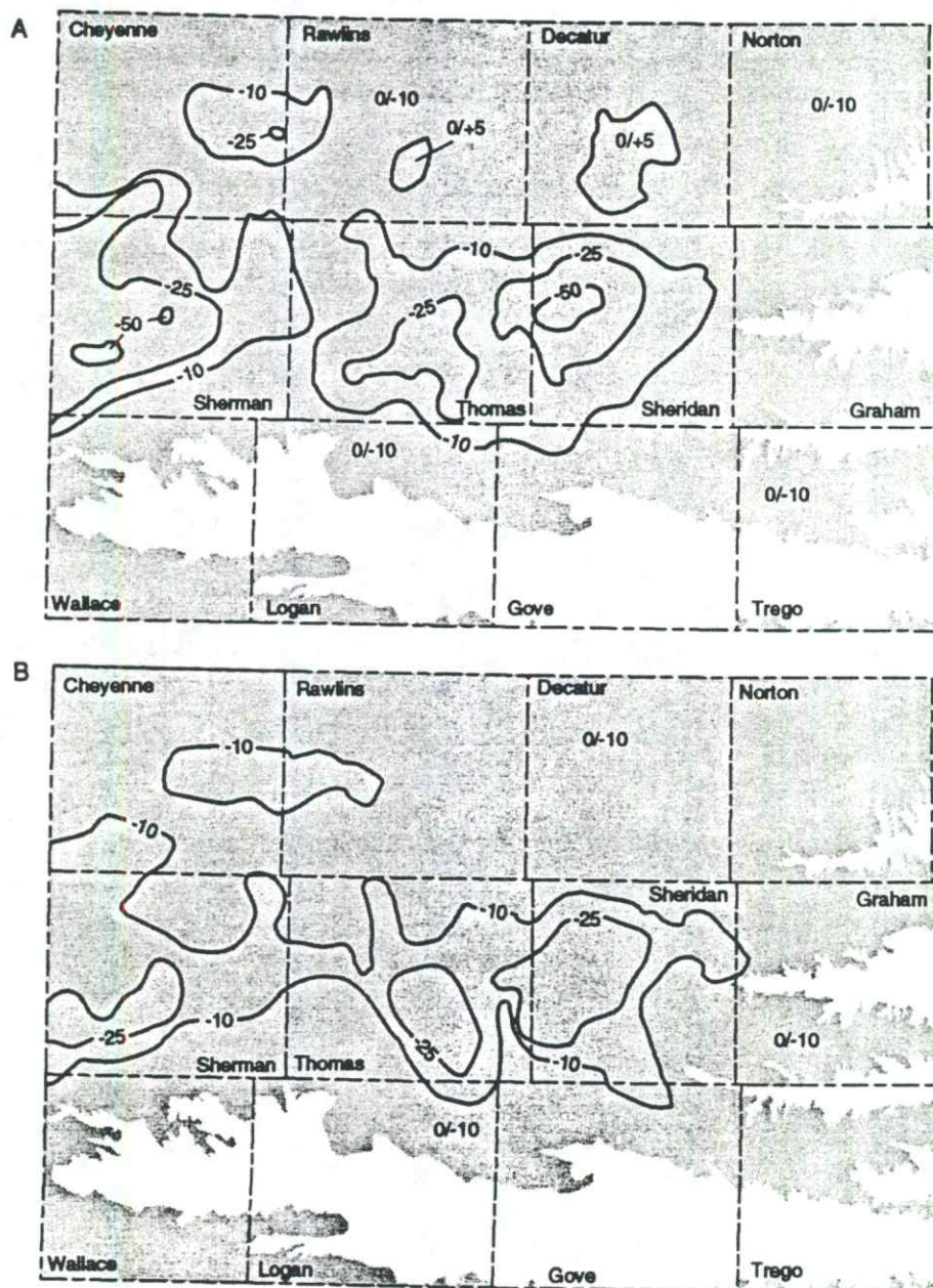
Figure 11. (A) Generalized water-level change (in feet) in region III, northwest Kansas, predevelopment to 1993. (B) Change (%) in saturated thickness in region III, northwest Kansas, predevelopment to 1993. (C, opposite ) Annual water-level change (in feet) in region III, northwest Kansas, for 1993.
