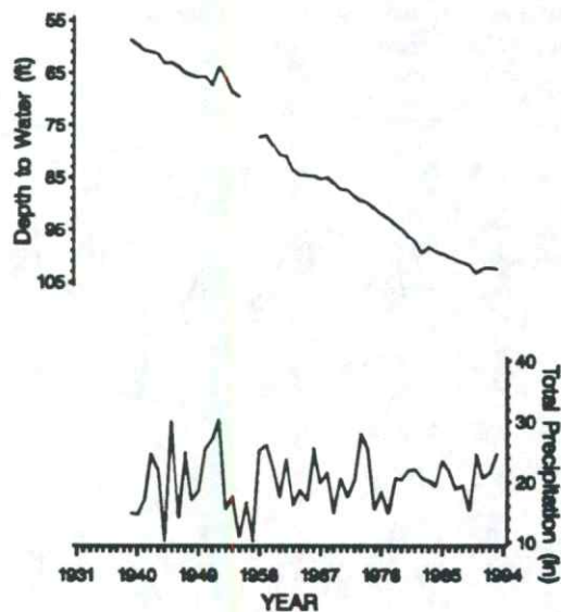
Figure 6. Water levels in Scott County well 20S 33W 09 BBB 01 [128 ft (39.0 m) deep, Ogallala Formation]. Compared to precipitation at Utica (station 14832804).
