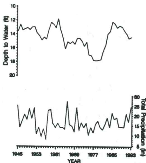
Figure 4. Water levels in Hamilton County well 23S 43W 21 ABA 01 [29 ft (8.8 m) deep, alluvial formation]. Compared to precipitation at Syracuse (station 14803807).
