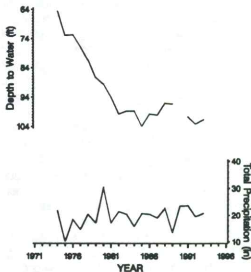
Figure 3. Water levels in Finney County well 24S 33W 28 DAA 01 [185 ft (56.4 m) deep, Pleistocene/Tertiary formations]. Compared to precipitation at the Garden City Experimental Station (station 14298007).
