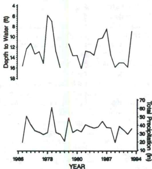
Figure 2. Relationship between precipitation and water level in Douglas County well 12S 20E 07 CBC 01 [29 ft (9 m) deep; Pleistocene formation]. Precipitation records are from the Topeka WSFO Airport (station 14816706).
