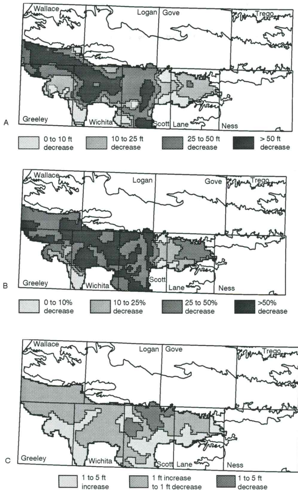
FIGURE 10—GROUND-WATER CHANGES IN THE AREA OF THE HIGH PLAINS AQUIFER IN REGION II, WEST-CENTRAL KANSAS. See fig. 11 for adjacent areas to the north, and fig. 9 for adjacent areas to the south. (A) Generalized water-level changes (in ft), predevelopment to 1994. (B) Change (%) in saturated thickness, predevelopment to 1994. (C) Annual water-level change (in ft), 1993-94.
