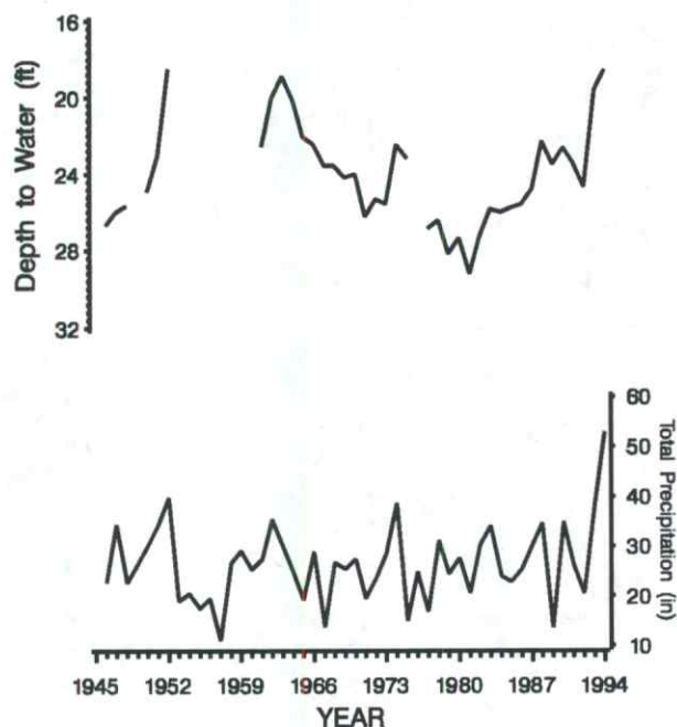
FIGURE 5—COMPARISON OF PRECIPITATION AT CAWKER CITY (STATION 14137102) WITH WATER LEVELS IN OSBORNE COUNTY WELL 06S-12W-23-CDC-01 [30 ft (9.1 m) deep, alluvial formation].
