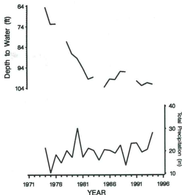
FIGURE 3—WATER LEVELS IN FINNEY COUNTY WELL 24S-33W-28-DAA-01 [185 ft (56.4 m) deep, Pleistocene/Tertiary formations]. Compared to precipitation at the Garden City Experimental Station (station 14298007).
