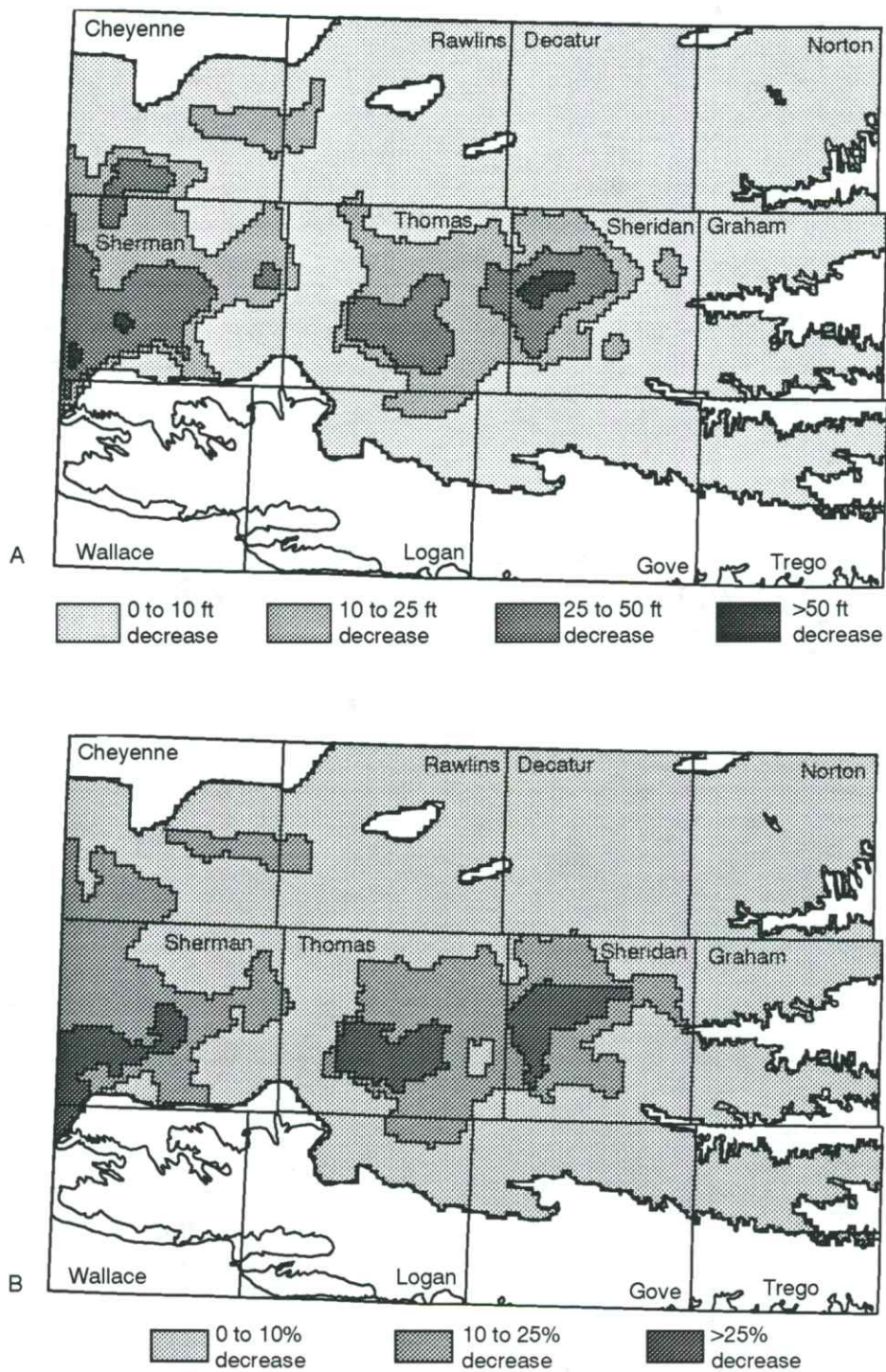
FIGURE 11—GROUND-WATER CHANGES IN THE AREA OF THE HIGH PLAINS AQUIFER IN REGION III, NORTHWEST KANSAS. See fig. 10 for adjacent areas to the south. (A) Generalized water-level changes (in ft), predevelopment to 1994. (B) Change (%) in saturated thickness, predevelopment to 1994. (C, following page) Annual water-level change (in ft), 1993–94.
