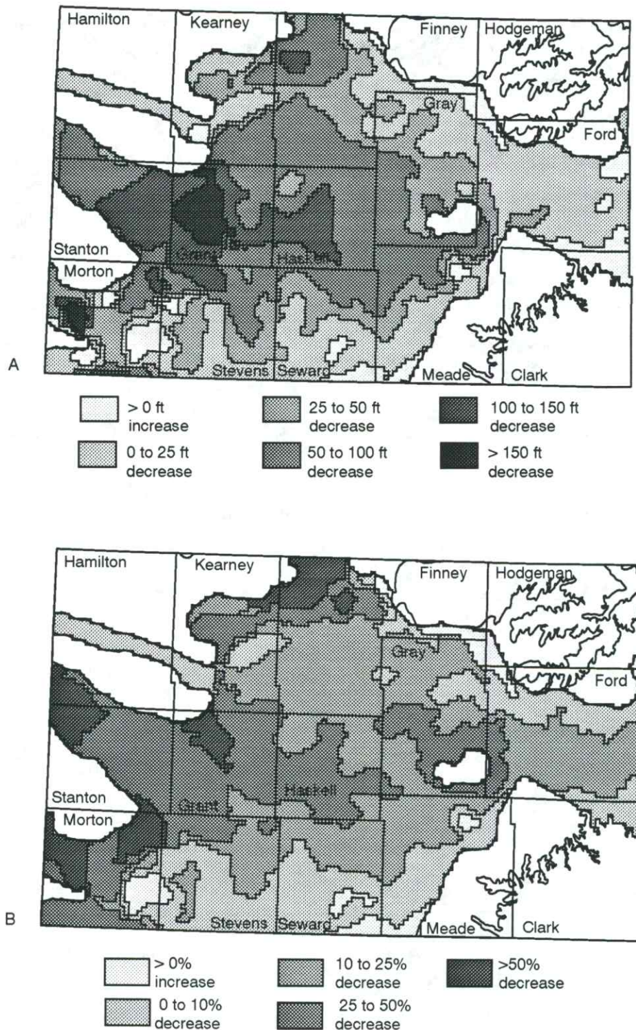
FIGURE 9—GROUND-WATER CHANGES IN THE AREA OF THE HIGH PLAINS AQUIFER IN REGION I, SOUTHWEST KANSAS. See fig. 10 for adjacent areas to the north, and fig. 12 for adjacent areas to the east. (A) Generalized water-level changes (in ft), predevelopment to 1994. (B) Change (%) in saturated thickness, predevelopment to 1994. (C, following page) Annual water-level change (in ft), 1993–94.
