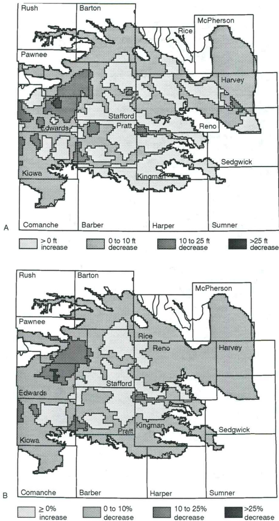
FIGURE 12—GROUND-WATER CHANGES IN THE AREA OF THE HIGH PLAINS AQUIFER IN REGION V, SOUTH-CENTRAL KANSAS. See fig. 9 for adjacent areas to the west. (A) Generalized water-level changes (in ft), predevelopment to 1994. (B) Change (%) in saturated thickness, predevelopment to 1994. (C, following page) Annual water-level change (in ft), 1993–94.
