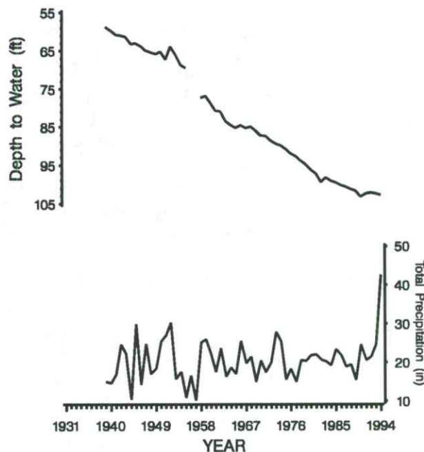
FIGURE 6—WATER LEVELS IN SCOTT COUNTY WELL 20S-33W-09-BBB-01 [128 ft (39.0 m) deep, Ogallala Formation]. Compared to precipitation at Utica (station 14832804).
