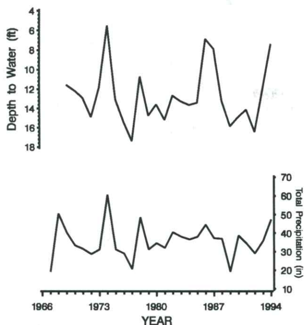
FIGURE 2—RELATIONSHIP BETWEEN PRECIPITATION AND WATER LEVEL IN DOUGLAS COUNTY WELL 12S-20E-07-CBC-01 [29 ft (9 m) deep; Pleistocene formation]. Precipitation records are from the Topeka WSFO Airport (station 14816706).
