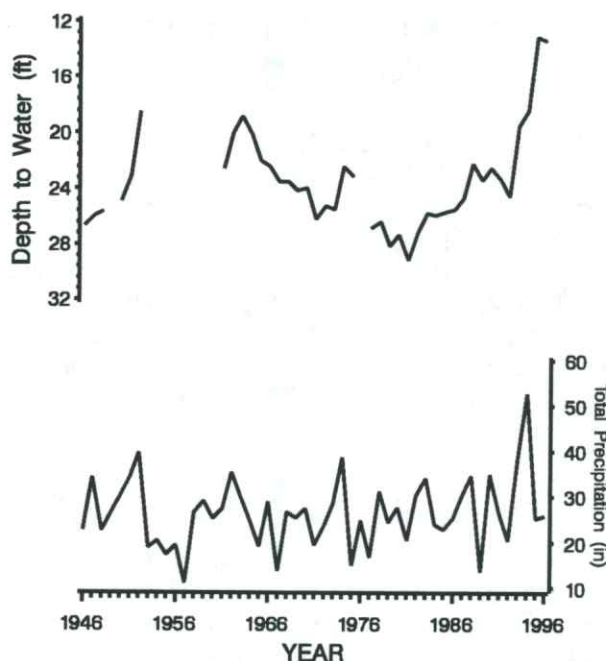
FIGURE 5—Depth to water in Osborne County, well 06S-12W-23-CDC-01 [30 ft (9.1 m) deep; alluvial formation], and precipitation at Cawker City (station 14137102).
