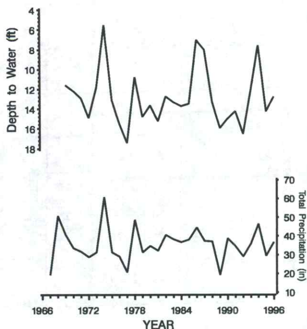
FIGURE 2—Depth to water in Douglas County, well 12S-20E-07-CBC-01 [29 ft (8.8 m) deep; Pleistocene formation], and precipitation at Topeka WSFO Airport (station 14816706).
