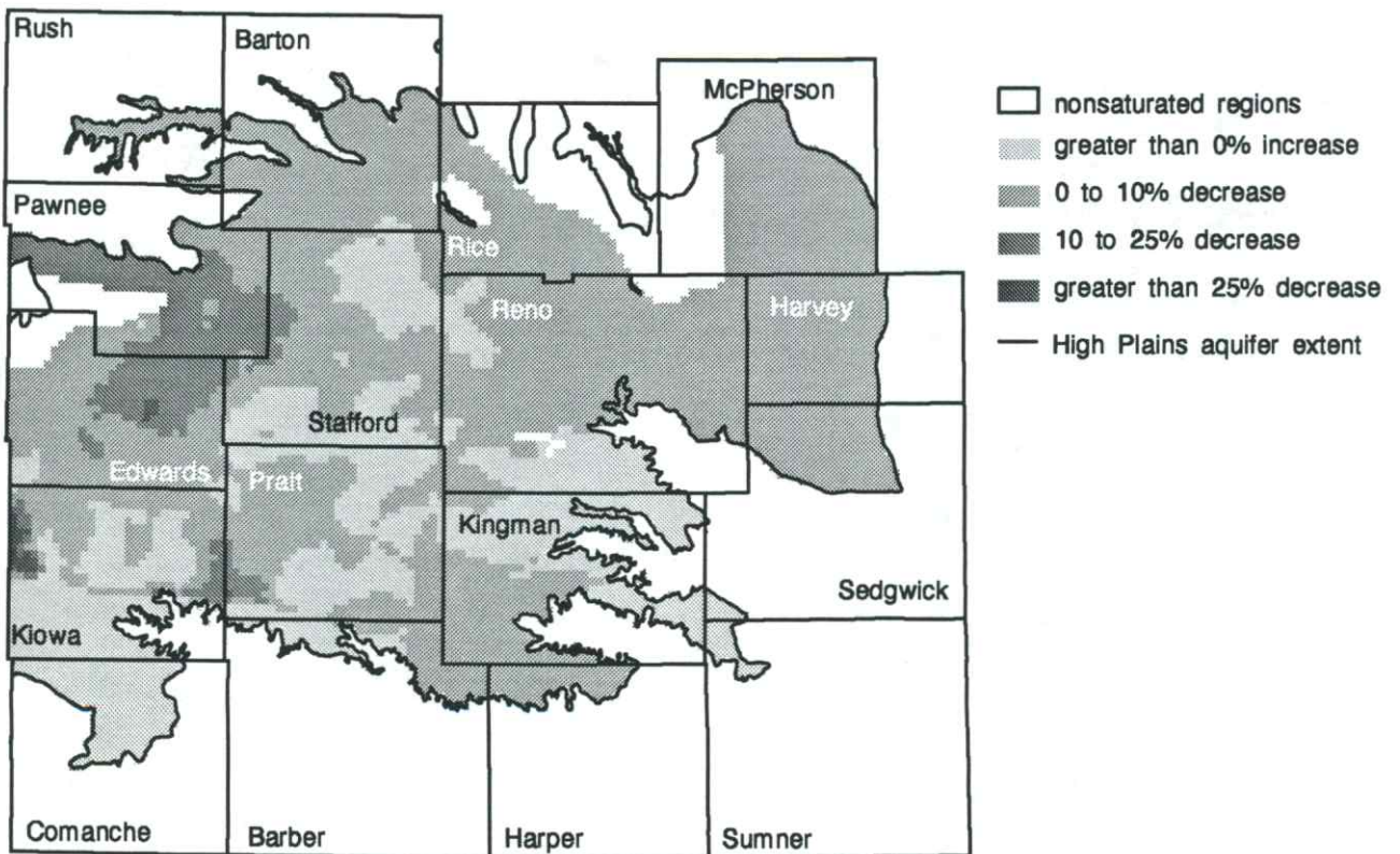
FIGURE 12—Ground-water changes in the area of the High Plains aquifer in Region V, south-central Kansas. See fig. 9 for adjacent areas to the west. (A) Generalized water-level changes (in ft), predevelopment to 1996. (B) Change (%) in saturated thickness, predevelopment to 1996. (C, following page.)
