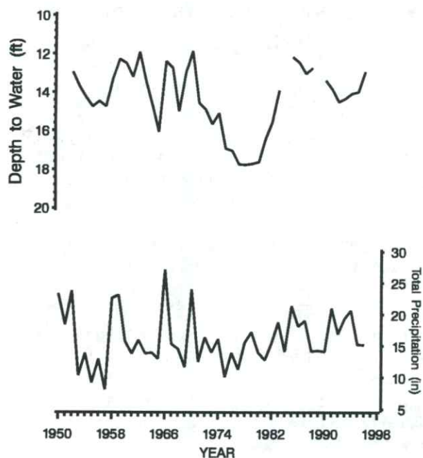
FIGURE 4—Depth to water in Hamilton County, well 23S-43W-21-ABA-01 [29 ft (8.8 m) deep; alluvial formation], and precipitation at Syracuse (station 14803807).
