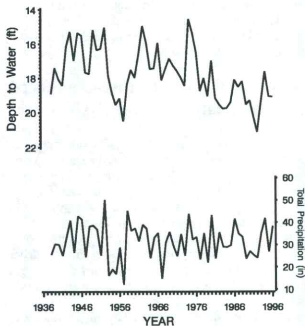
FIGURE 7—Depth to water in Sedgwick County, well 25S-01W-26-DBD-01 [54 ft (16 m) deep; Pleistocene alluvial formation], and precipitation at Mount Hope (station 14553908).
