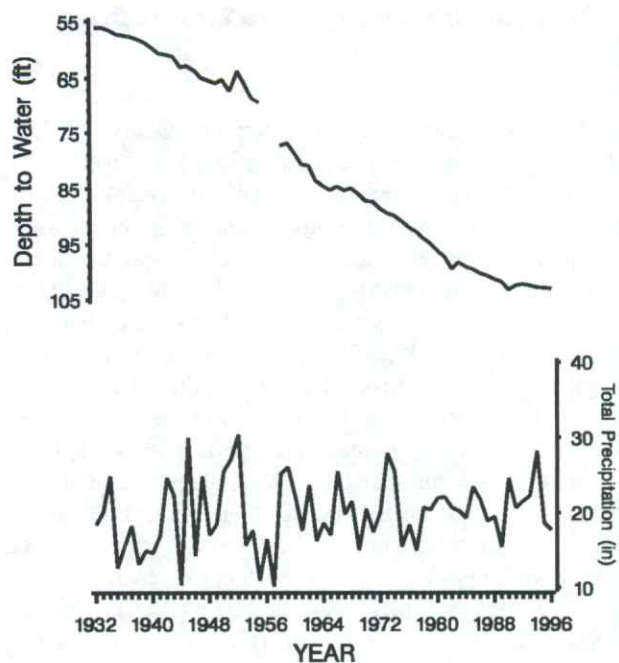
FIGURE 6—Depth to water in Scott County, well 20S-33W-09-BBB-01 [128 ft (39.0 m) deep; Ogallala Formation], and precipitation at Scott City (station 14727104).
