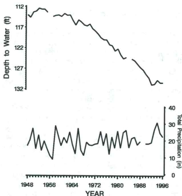
FIGURE 8 (left)—Depth to water in Thomas County, well 08S-34W-01-BAC-01 [160 ft (48.8 m) deep; Ogallala Formation], and precipitation at Colby 1 SW (station 14169901).
