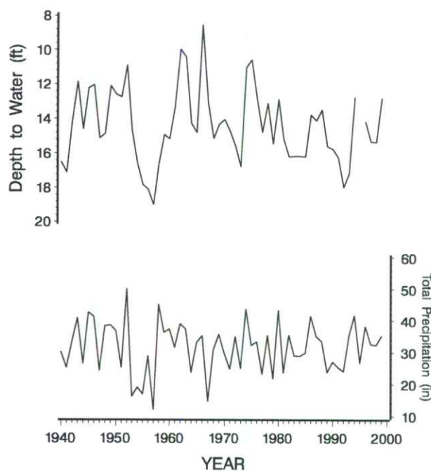
FIGURE 7—DEPTH TO WATER IN SEDGWICK COUNTY, well 25S–01W–14–DDD–01 (30 ft [9.8 m] deep; alluvial aquifer), and precipitation at Mount Hope (station 14553908).
