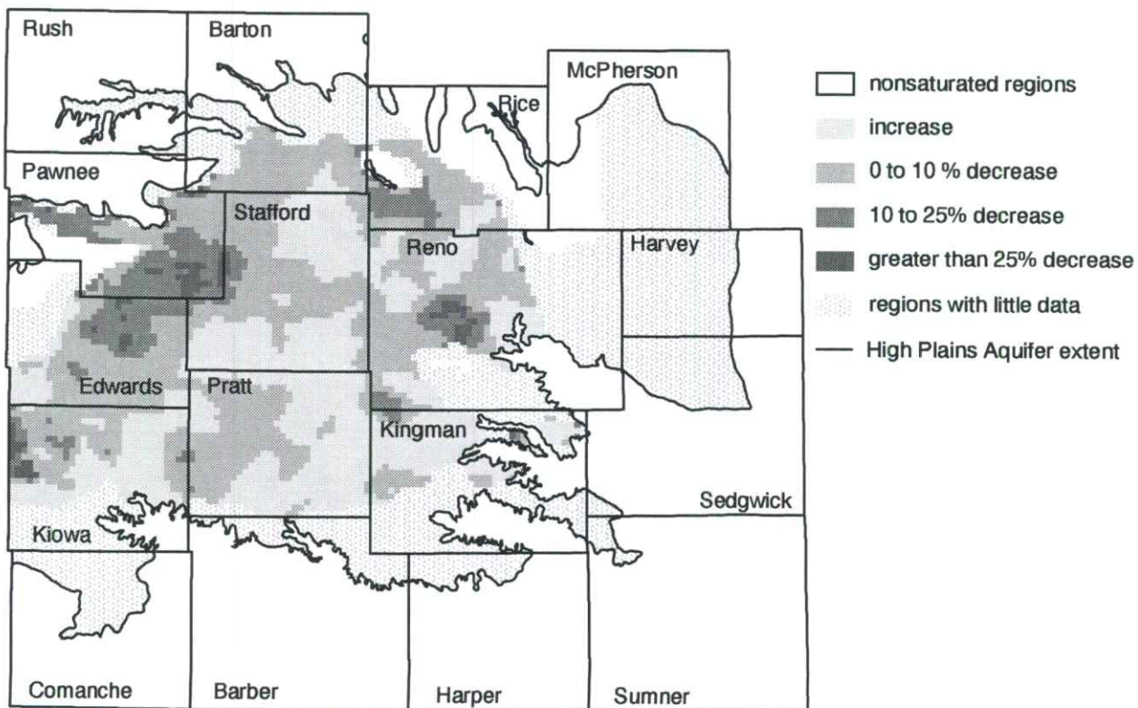
FIGURE 12 (above and next page)—GROUND-WATER CHANGES IN THE AREA OF THE HIGH PLAINS AQUIFER IN REGION V, SOUTH-CENTRAL KANSAS. See fig. 9 for adjacent areas to the west. (A) Generalized water-level changes (ft), predevelopment to 1999. (B) Change in saturated thickness (%), predevelopment to 1999. (C) Annual water-level change (ft), 1998–99.
