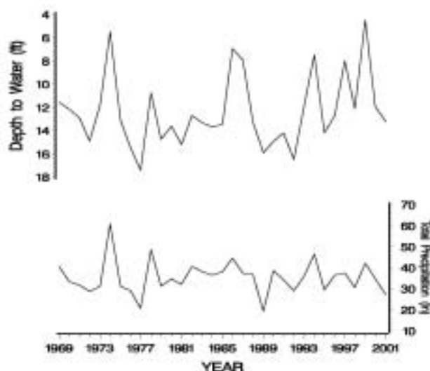
FIGURE 2. Depth to water in Douglas County, well 12S-20E-07-CBC-01 [29 ft (8.8 m) deep; alluvial aquifer], and precipitation at Topeka WSFO airport (station 14816706).
