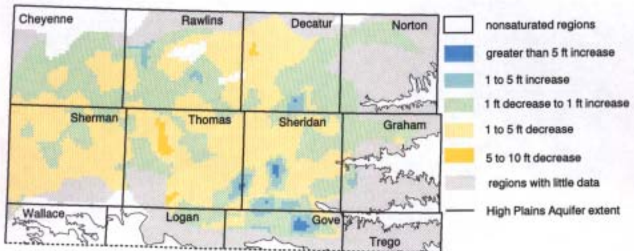
FIGURE 11C. Annual water-level change (ft), 2000-2001.
