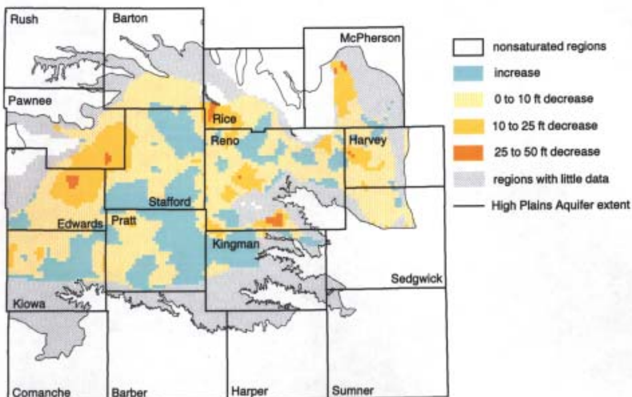
FIGURE 12A. Ground-water changes in the area of the High Plains aquifer in Region V, south-central Kansas. See fig. 9 for adjacent areas to the west. Generalized water-level changes (ft), predevelopment to 2001.
