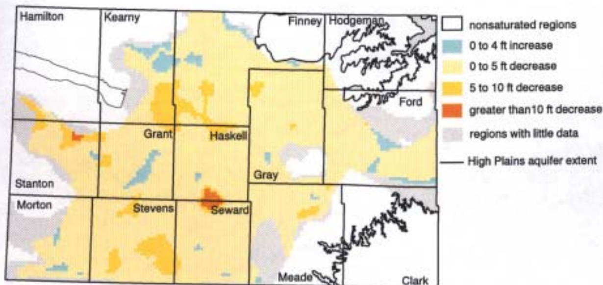
FIGURE 9C. Annual water-level change (ft), 2000-2001.
