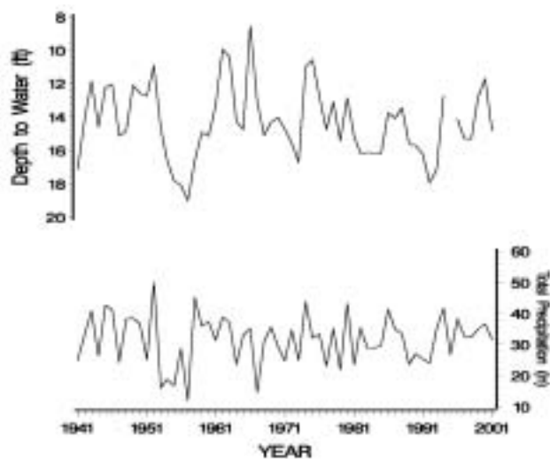
FIGURE 7. Depth to water in Sedgwick County, well 25S-01W-14-DDD-01 [alluvial aquifer], and precipitation at Mount Hope (station 14553908).
