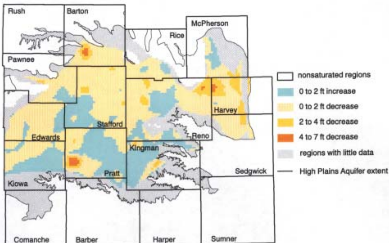
FIGURE 12C. Annual water-level change (ft), 2000-2001.
