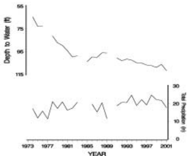
FIGURE 3. Depth to water in Finney County, well 24S-33W-28-DAA-01 [350 ft (107 m) deep; High Plains aquifer], and precipitation at Garden City Experimental Station (station 14298007).
