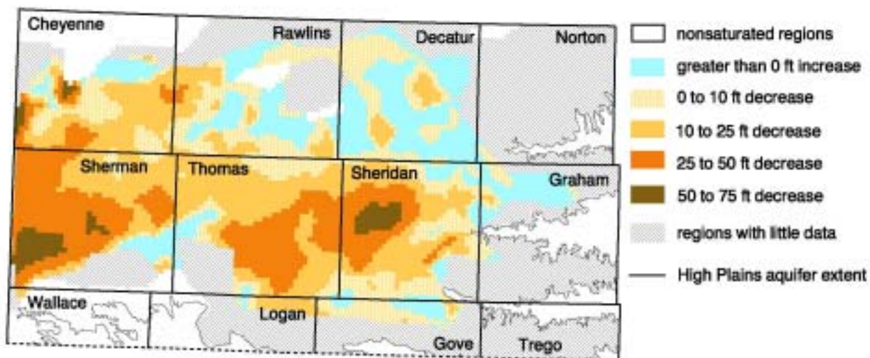
FIGURE 11A. Ground-water changes in the area of the High Plains aquifer in Region III, northwestern Kansas. See fig. 10 for adjacent areas to the south. Generalized water-level changes (ft), predevelopment to 2001.
