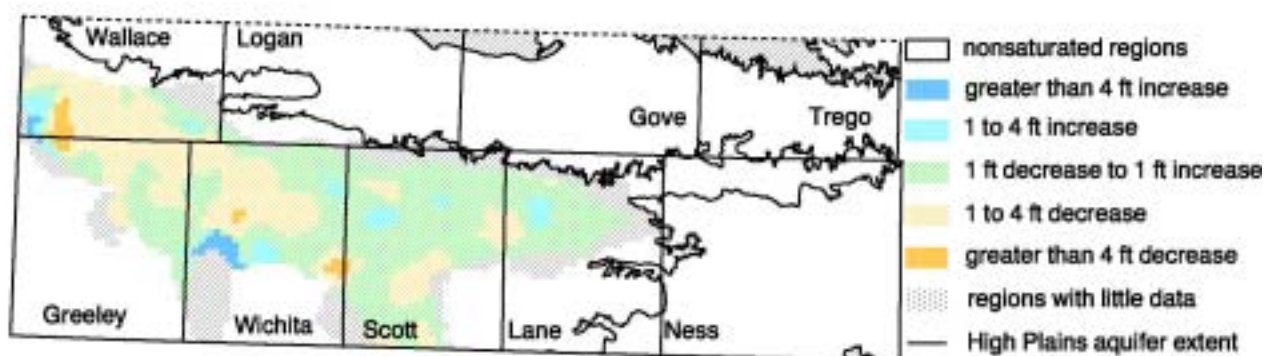
FIGURE 10C. Annual water-level change (ft), 2000-2001.
