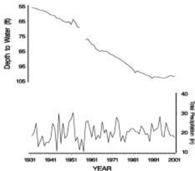
FIGURE 6. Depth to water in Scott County, well 20S-33W-09-BBB-01 [128 ft (39.0 m) deep; High Plains aquifer], and precipitation at Scott City (station 14727104).
