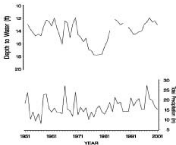
FIGURE 4. Depth to water in Hamilton County, well 23S-43W-21-ABA-01 [29 ft (8.8 m) deep; alluvial aquifer], and precipitation at Syracuse (station 14803807).
