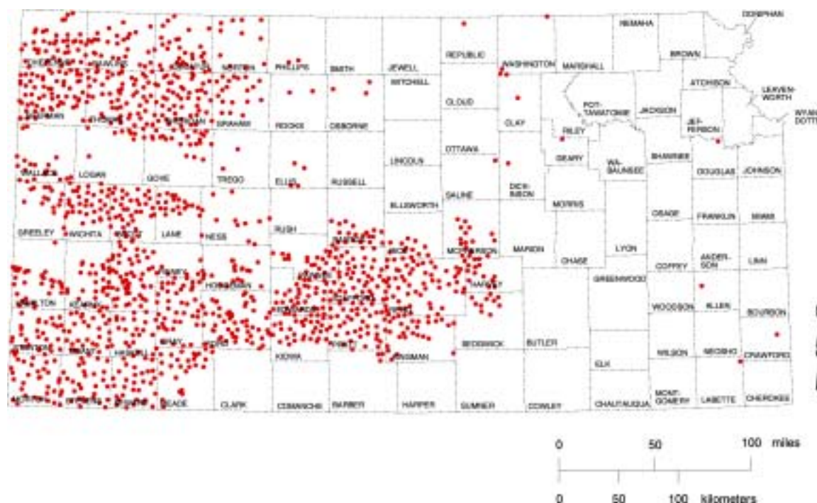
FIGURE 1B. Distribution of ground-water level observation wells measured for the 2001 water-level census.
