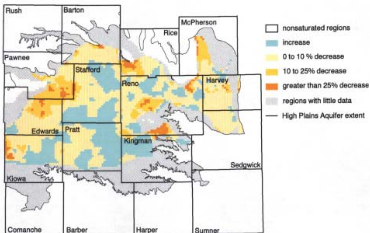
FIGURE 12B. Change in saturated thickness (%), predevelopment to 2001.
