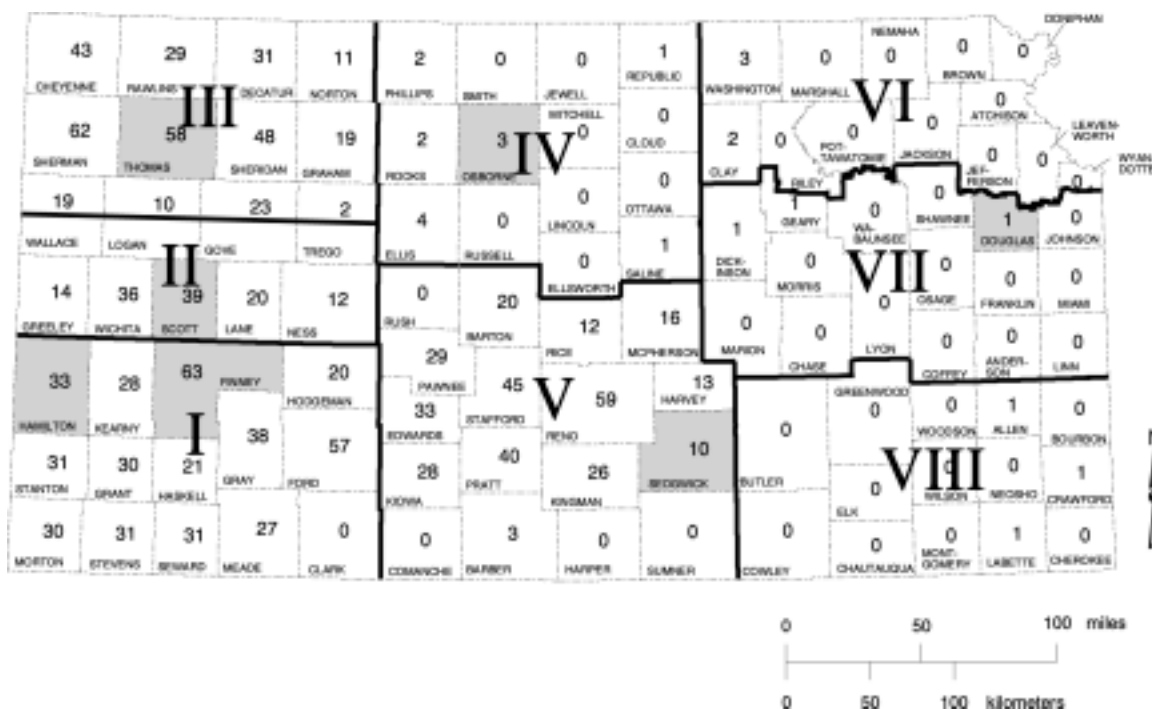
FIGURE 1A. Number of ground-water level observation wells measured in each county for the 2001 water-level census. Shaded counties are those for which precipitation graphs and well hydrographs are presented in the text.
