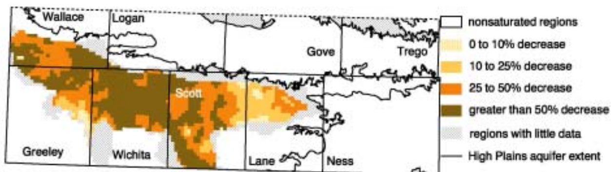
FIGURE 10B. Change in saturated thickness (%), predevelopment to 2001.
