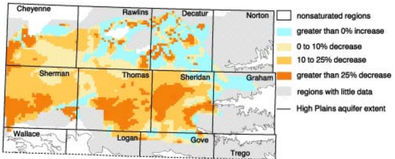
FIGURE 11B. Change in saturated thickness (%), predevelopment to 2001.
