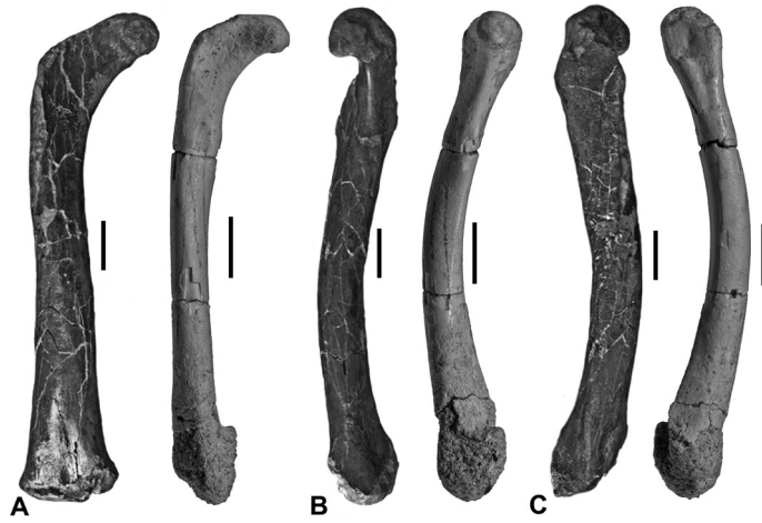
Figure 9. Dakotaraptor holotype (PBMNH.P.10.113.T) femur (left) compared with Mahakala omnigovae (IGM 100/1033; right, reversed). Femora shown in (A) dorsal, (B) medial, and (C) lateral views. The femur of Dakotaraptor retains the elongate and gracile proportions of the smaller raptor despite Dakotaraptor 's much larger size. The two femora also share a similar low-angle connection between the femoral head and the shaft, and a noticeable anteroposterior bow to the shaft. Dakotaraptor scale bars = 6 cm; Mahakala scale bars = 1 cm. Mahakala images courtesy Mike Ellington and Mark Norell, AMNH.
