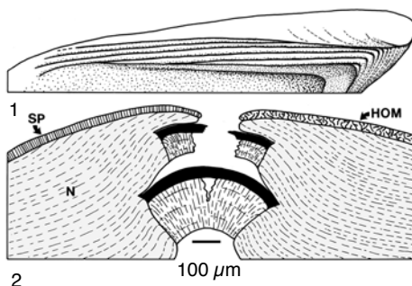
FIG. 202. Upper Carboniferous myalinid Septimyalina perattenuata (MEEK & HAYDEN, 1858), diagram based on specimen from Magoffin Member, Breathitt Formation, Milepost 55 on the Daniel Boone Parkway (UNC 13664). 1, Internal view of left hinge showing multiple ligamental groove/ridge couplets in opisthodontic, low-angle, duplivincular ligament; figure width is about 15 mm; 2, transverse section through posterior part of ligament, with lamellar sublayers restored as solid black bands; SP, calcitic regular simple prismatic outer shell layer; HOM, calcitic homogeneous outer shell layer; N, nacre (adapted from Carter, 2004, fig. 2.1–2.2).
