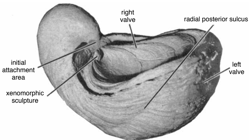
FIG. 127. Liassic, Lower Jurassic gryphaeid Gryphaea ( Gryphaea ) arcuata LAMARCK, 1801, England, illustrating gryphaeiform shell shape, maximum figure dimension 46 mm (adapted from Stenzel, 1971, fig. J74.3e).
