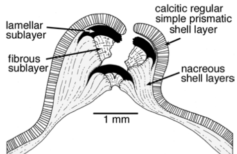
FIG. 258. Reduced low-angle, opisthodontic duplivincular ligament as seen in upper Carboniferous pinnid Meekopinna americana (MEEK, 1867), Magoffin Member, Breathitt Formation, Milepost 55 along Daniel Boone Parkway, Hazard County, Kentucky (UNC 7352); transverse section through united valves (adapted from Carter, 2004, fig. 2.3).
