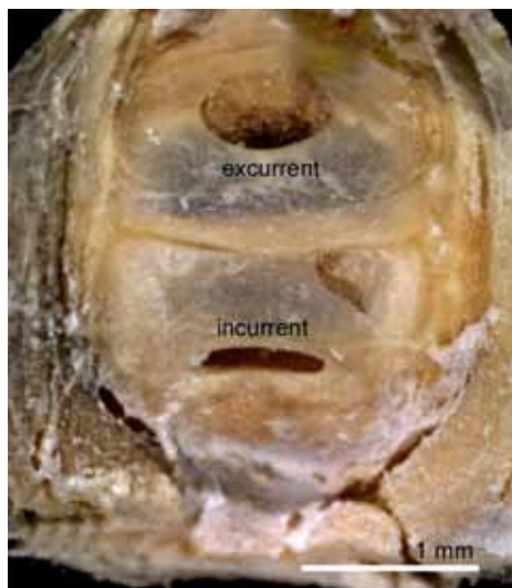
FIG. 32. Gastrochaenid Gastrochaena cuneiformis SPENGLER, 1783, Great Nicobar Island, Anadaman Sea (UNC, unnumbered specimen). Incurrent and excurrent basal siphonal diaphragms, viewed from mantle cavity toward base of siphons (Carter, new).
