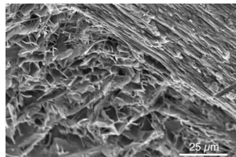
FIG. 55. Chalky microstructure (also called mocret) (lower left) in a vertical fracture through ostreoidan Crassostrea gigas (THUNBERG, 1793), eastern Atlantic (market specimen; N. Malchus no. s04661, stb 0241). Also visible is foliated shell layer (upper right) and a tubule or an endolithic boring (far right); shell exterior is toward upper right (Malchus, new).
