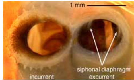
FIG. 287. Siphon tips of gastropod Lamychaena cordiformis (NEVILL & NEVILL, 1869), Ko Khai Nai Island, near Phuket, Andaman Sea, Thailand (UNC, unnumbered specimen), showing apical diaphragm on excurrent siphon tip (Carter, new).
