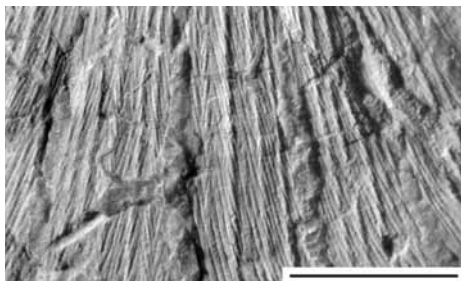
FIG. 114. Filous structure in transitional entoloidesid-propeamussiid Filamussium schaffhaeutli (WINKLER, 1859), Norian–Rhaetian, Upper Triassic, Kössener Schichten, Kotalm, Schweinsberg bei Miesbach, Germany. Composite external mold of left valve, also showing superimposed external radial costae and diagenetic calcite-filled imprints of internal, radial ribs; scale bar = 10 \mu m (adapted from Waller, 2006, fig. 7B).
