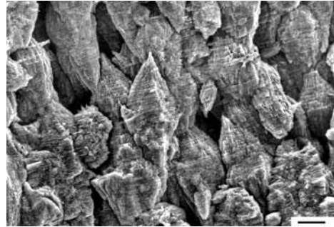
FIG. 312. Transitional granular/prismatic microstructure locally developed in aragonitic, otherwise prismatic outer shell layer of Recent hiatellid Cyrtodaria siliqua (SPENGLER, 1793), off Martha's Vineyard, Massachusetts (YPM 4995); SEM of a radial, vertical fracture; shell exterior is up and shell posterior is toward right; scale bar = 10 \mu m (Carter, new).
