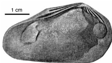
FIG. 3. Actinodont hinge dentition in left valve of middle Llandovery, lower Silurian actinodontid Actinodonta cuneata PHILLIPS, 1848; hinge teeth are actually continuously distributed below beak, contrary to this drawing. See also POJETA (1978, pl. 4,9–12) (Phillips, 1848).
