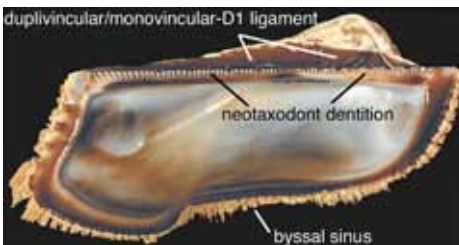
FIG. 25. Arcid Arcia imbricata BRUGUIÈRE, 1789, showing its subtrapezoidal shape, amphidetic, duplivincular/monovincular-D1 ligament, neotaxodont dentition, and byssal sinus; shell length several cm (adapted from Mikkelsen & Bieler, 2007).
