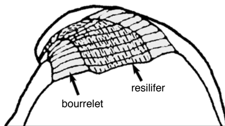
FIG. 129. Diagram of alivincular gyrostreoid ligament in Gyrostreia MIRKAMALOV, 1963 (adapted from Malchus, 1990, fig. 25b).
